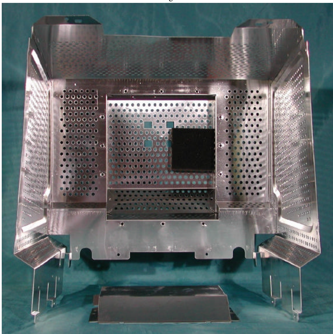
Shielding Cover
