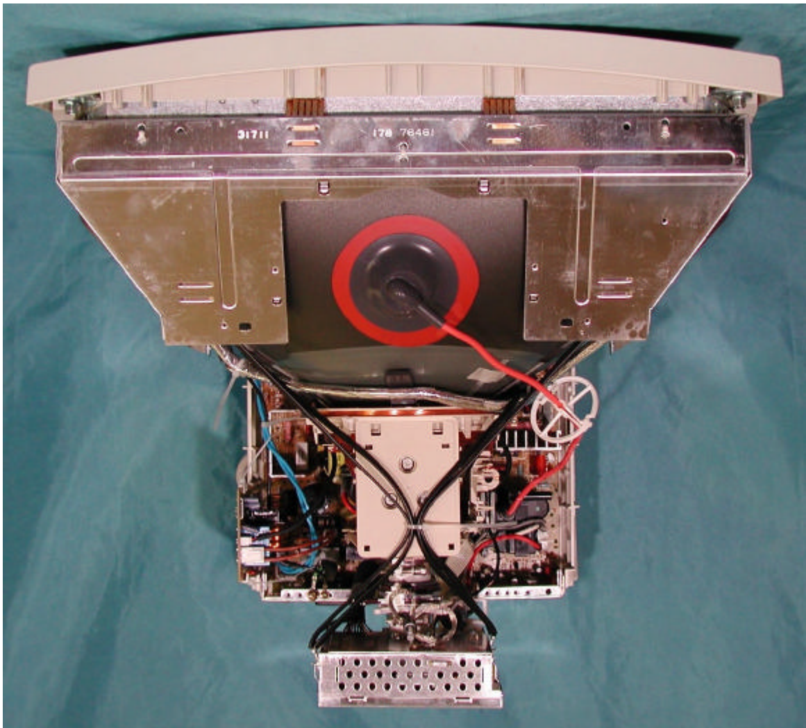
Top View w/o Shielding Cover
