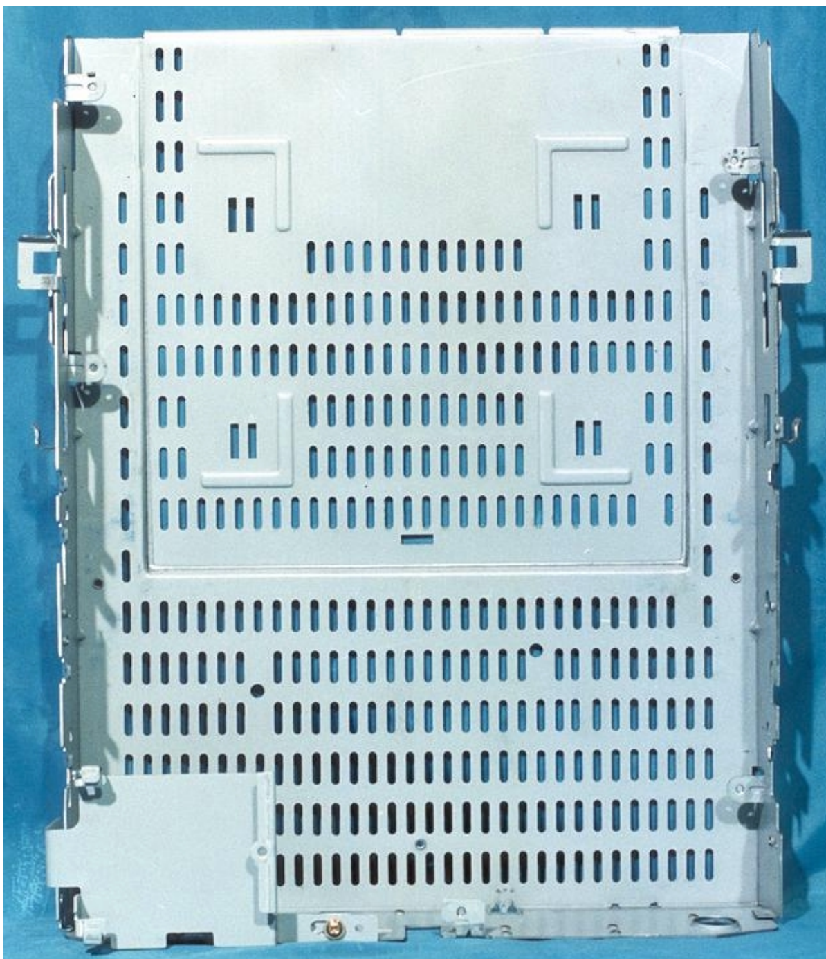
Shielding Plate
