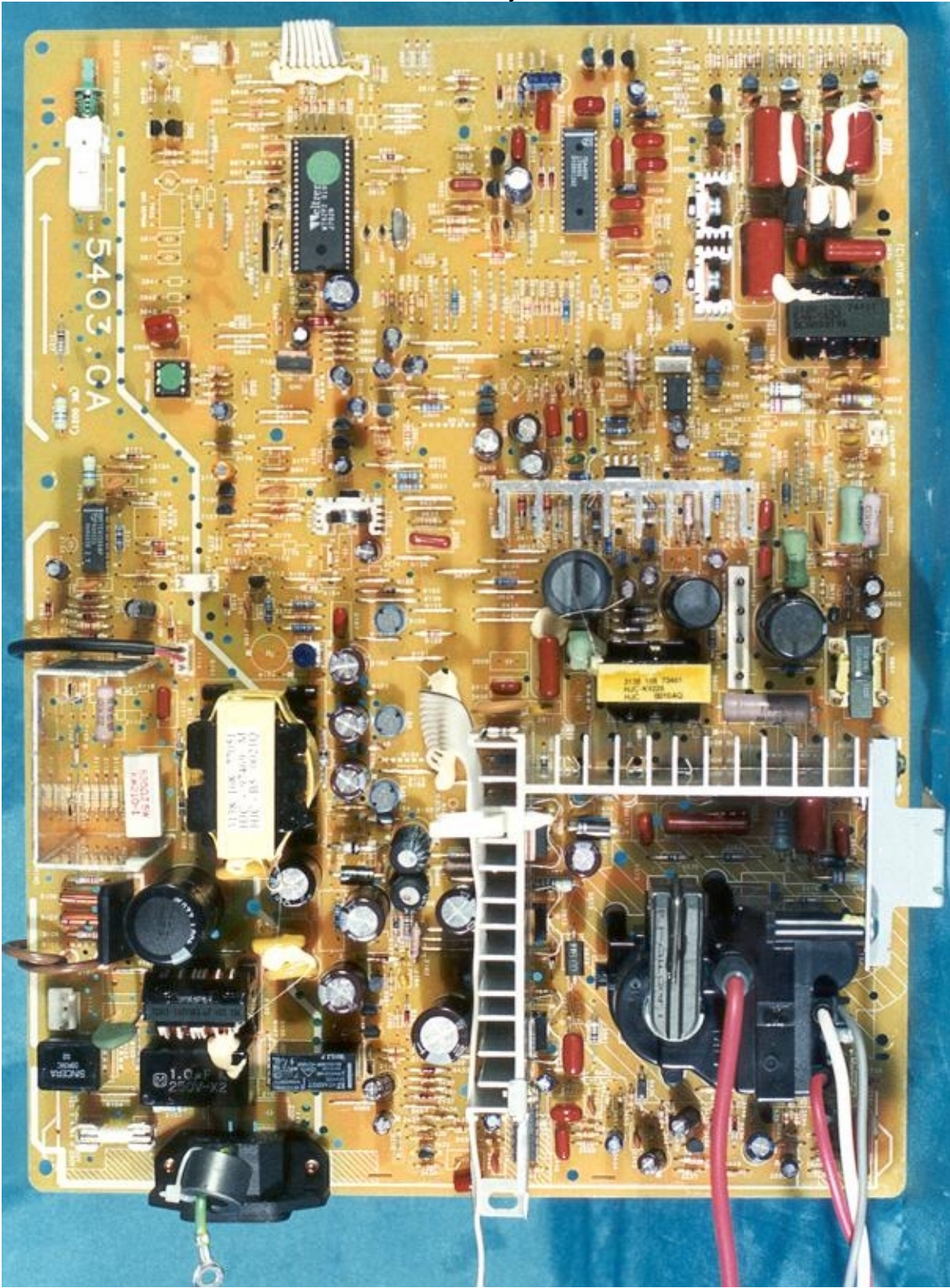
PCB Layout
