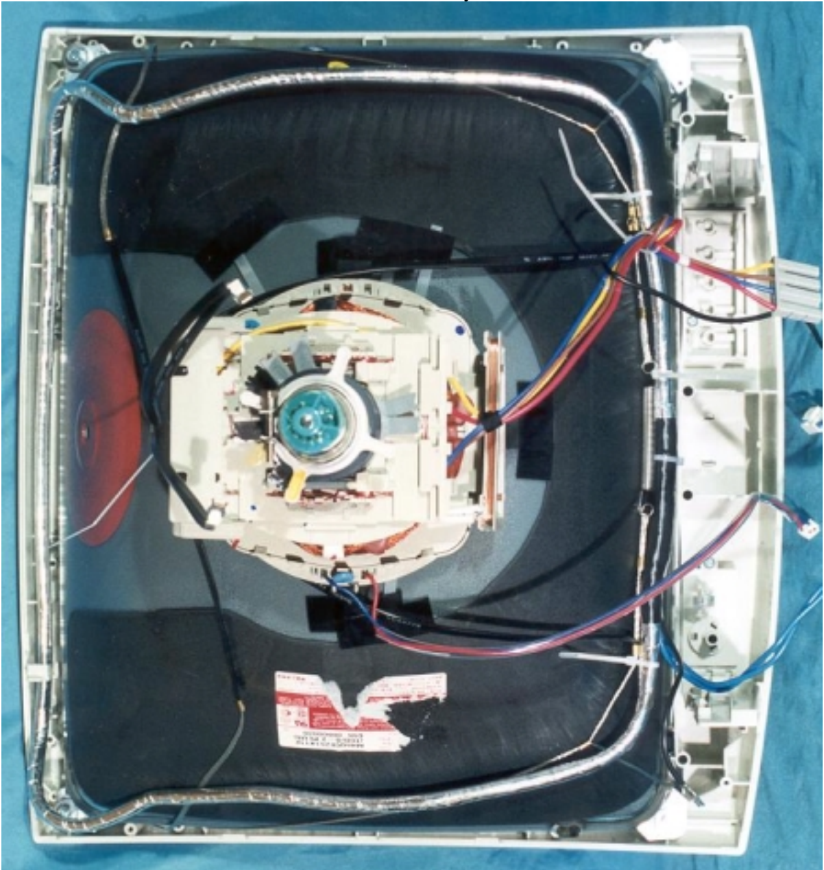
CRT Assembly
