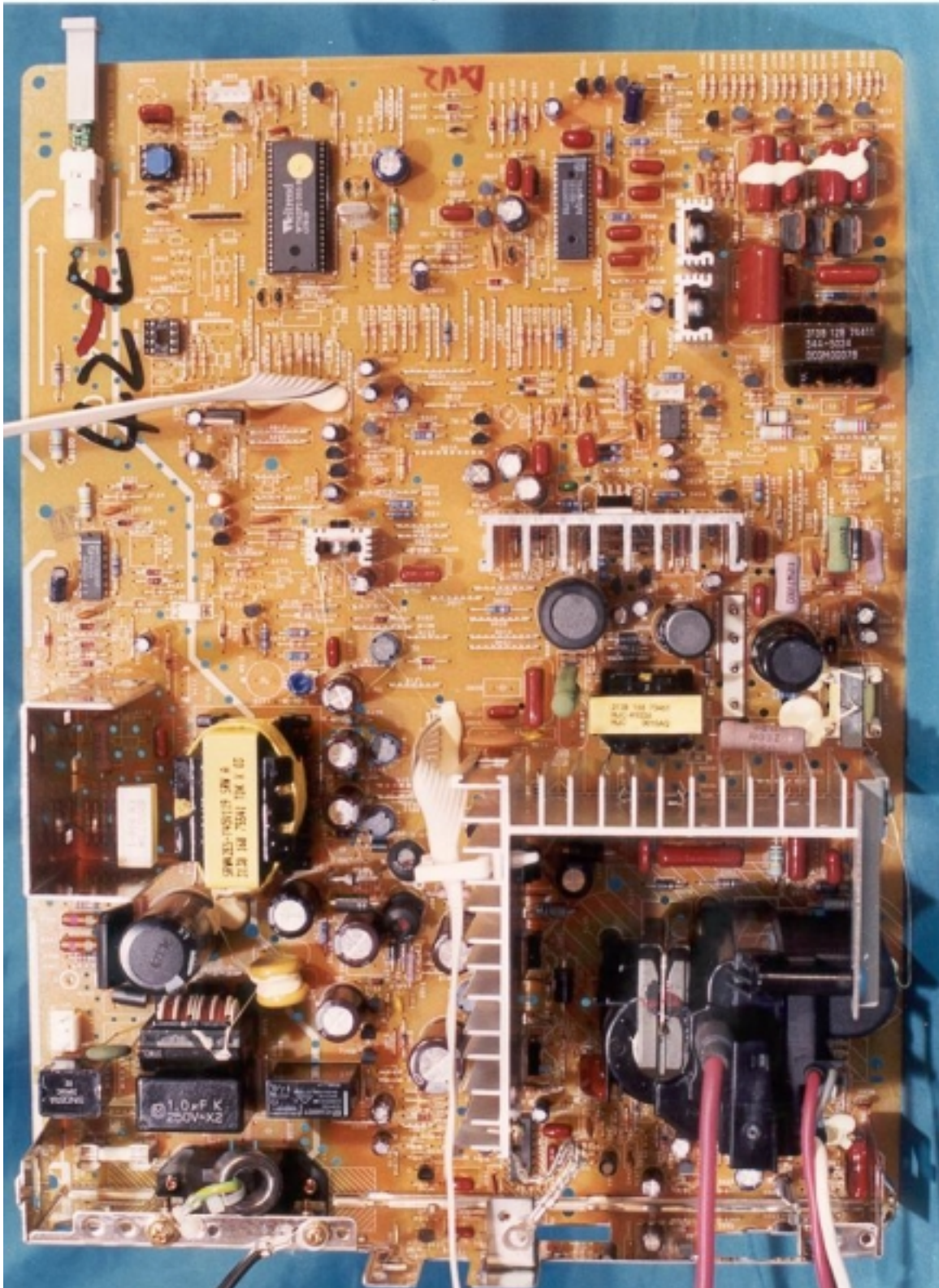
PCB Layout
