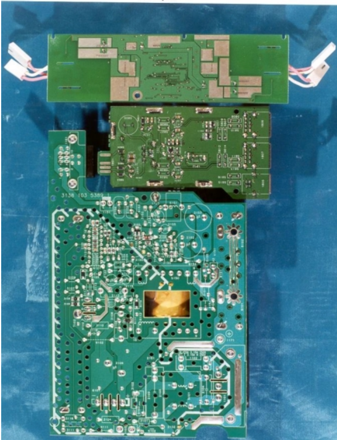
PCB Layout
