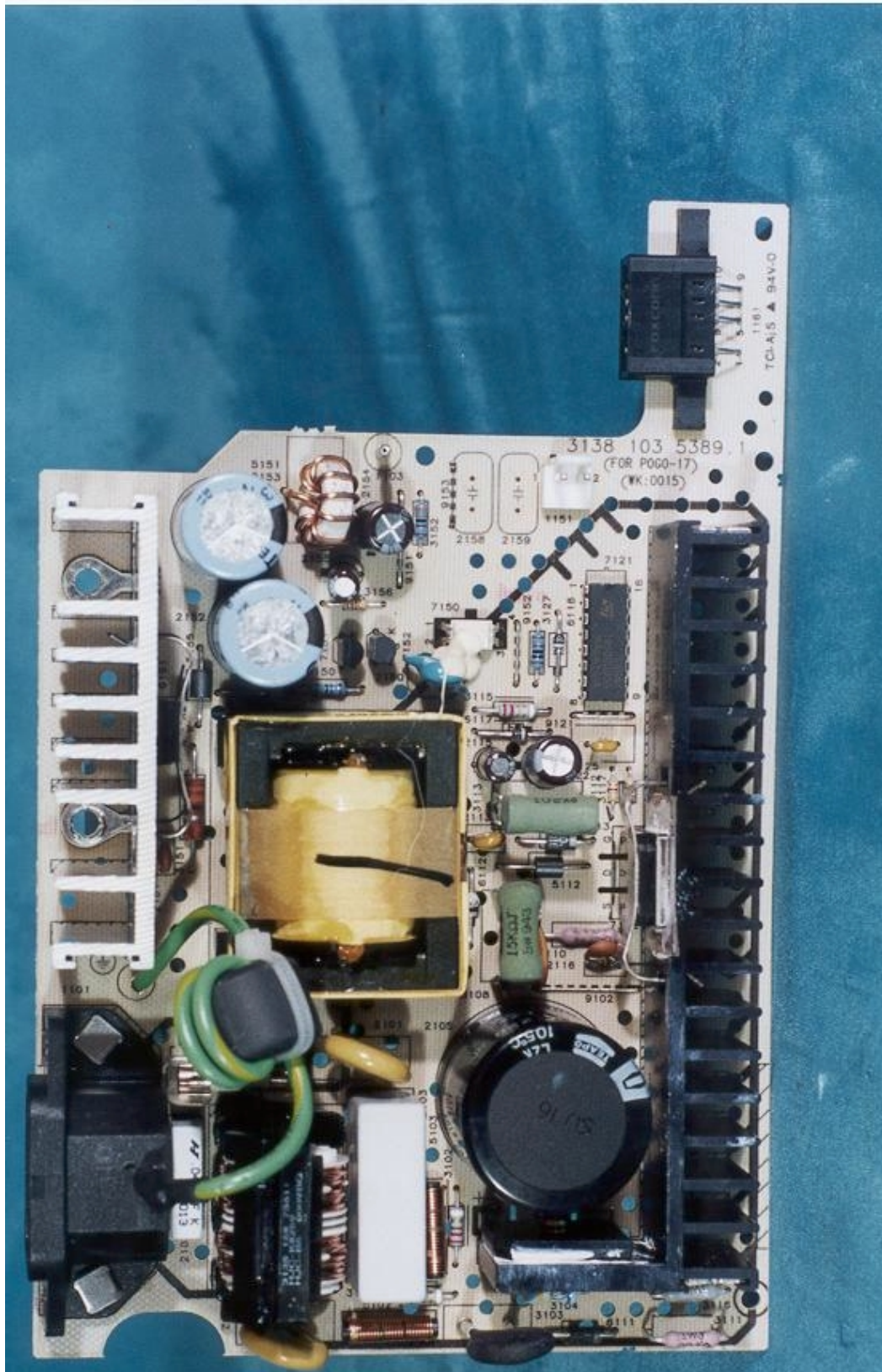
PCB Layout
