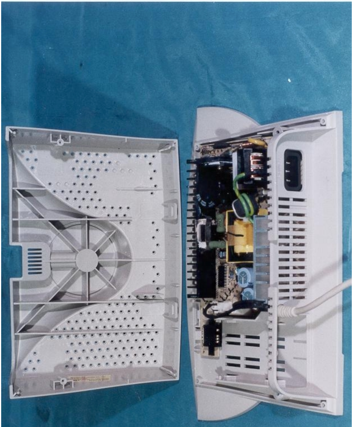
Power Supply
