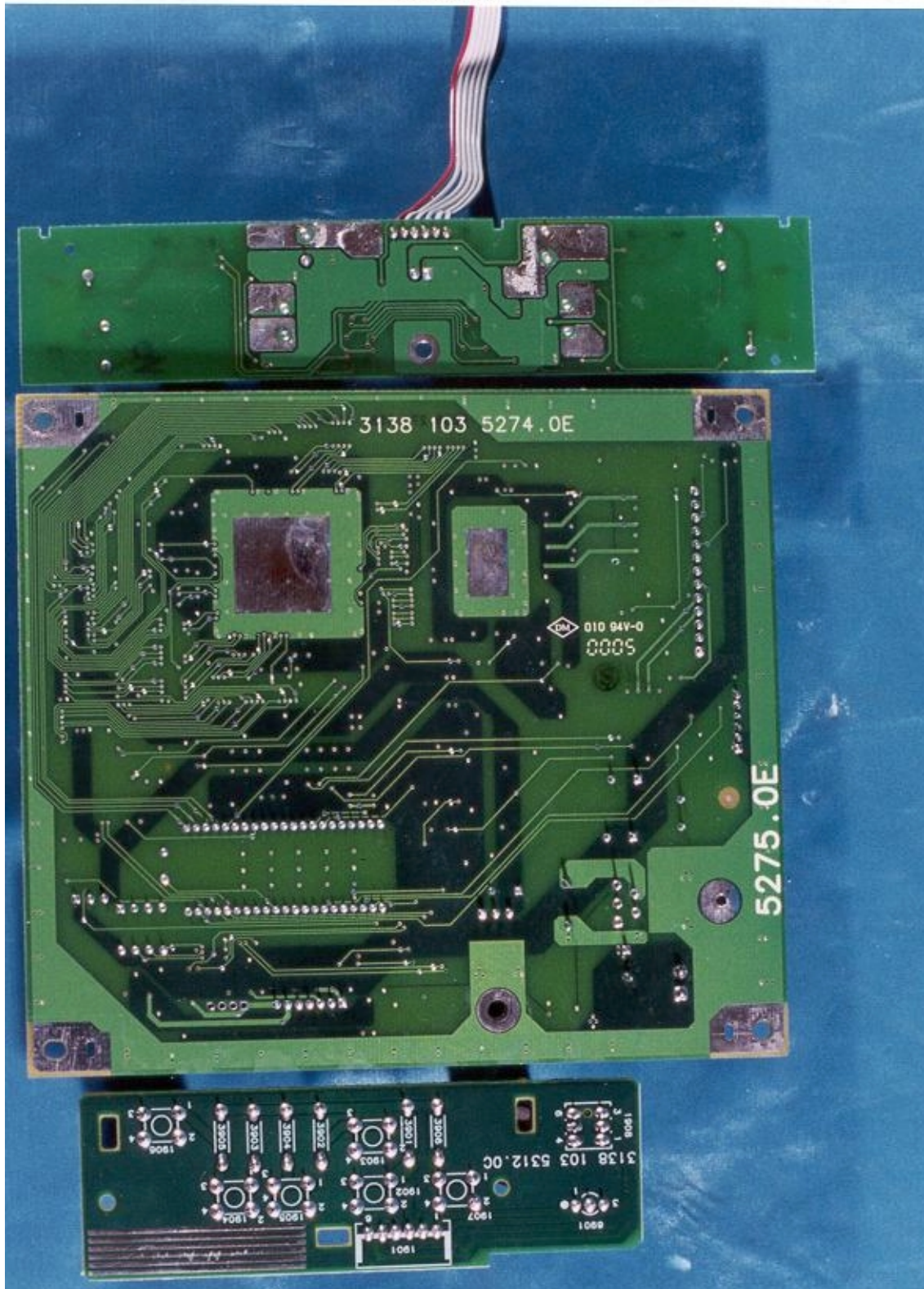
PCB Layout
