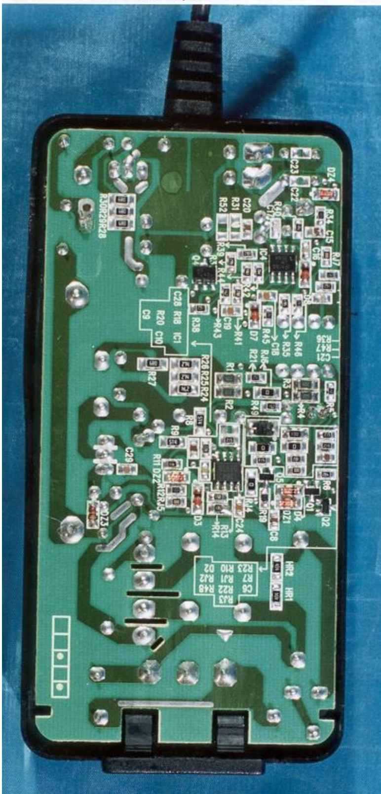
PCB Layout
