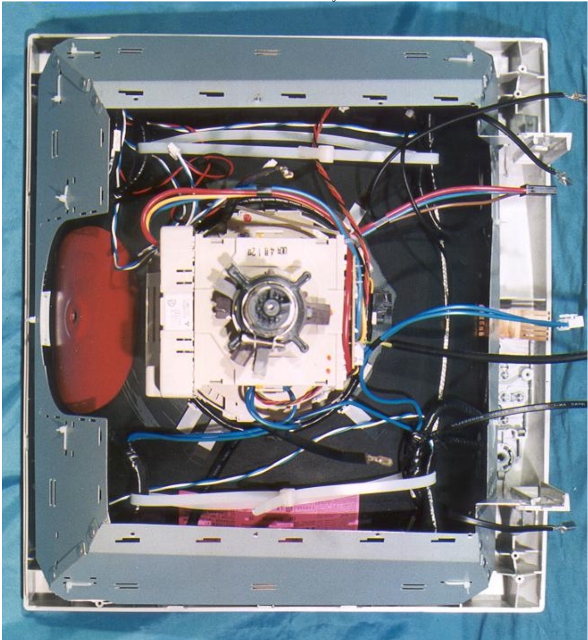
CRT Assembly
