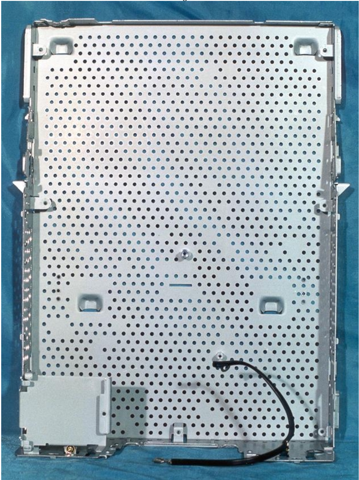
Shielding Plate
