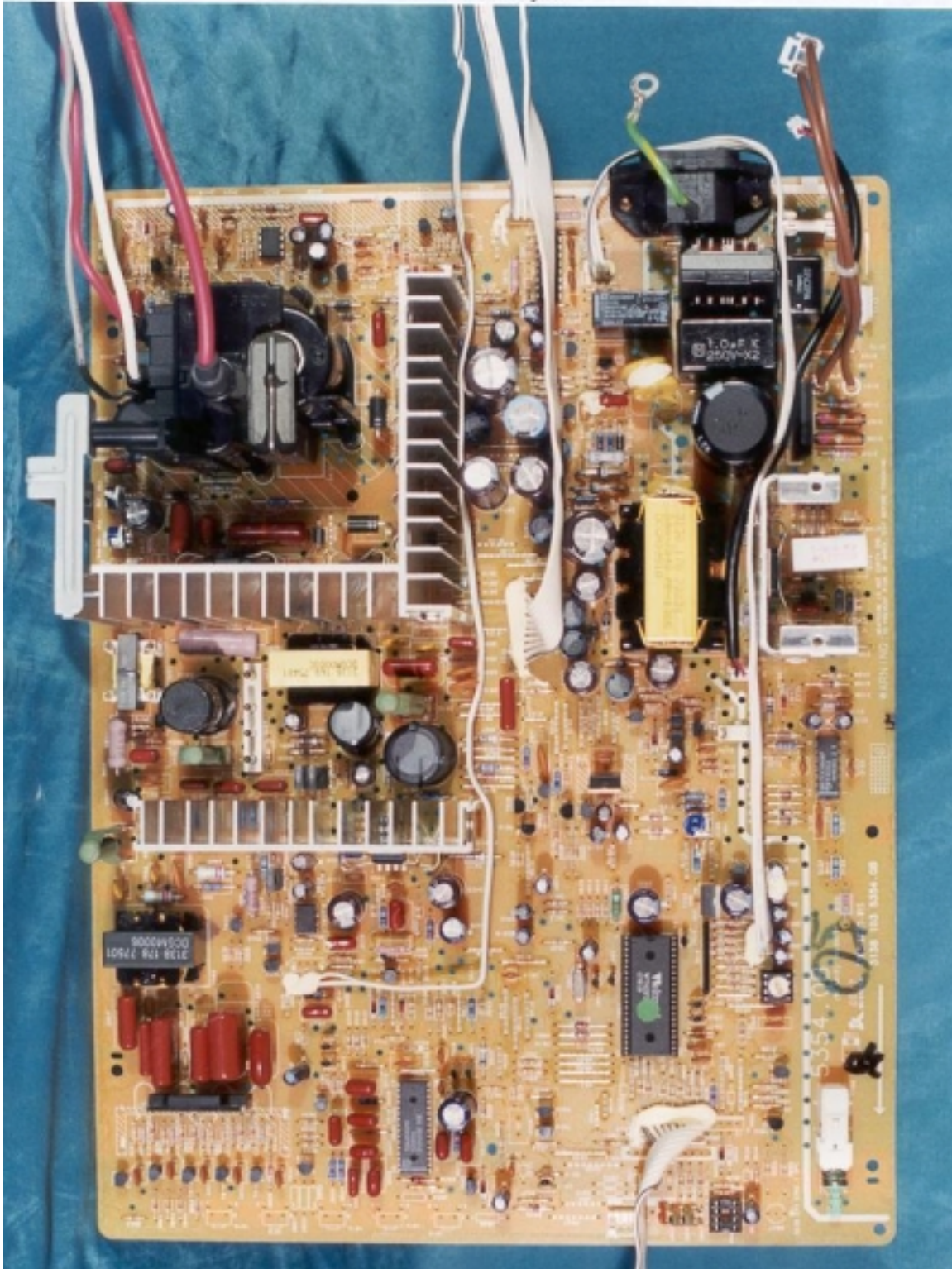
PCB Layout
