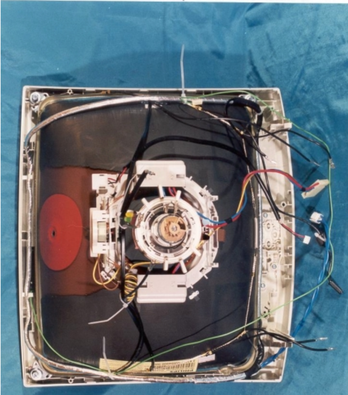
CRT Assembly
