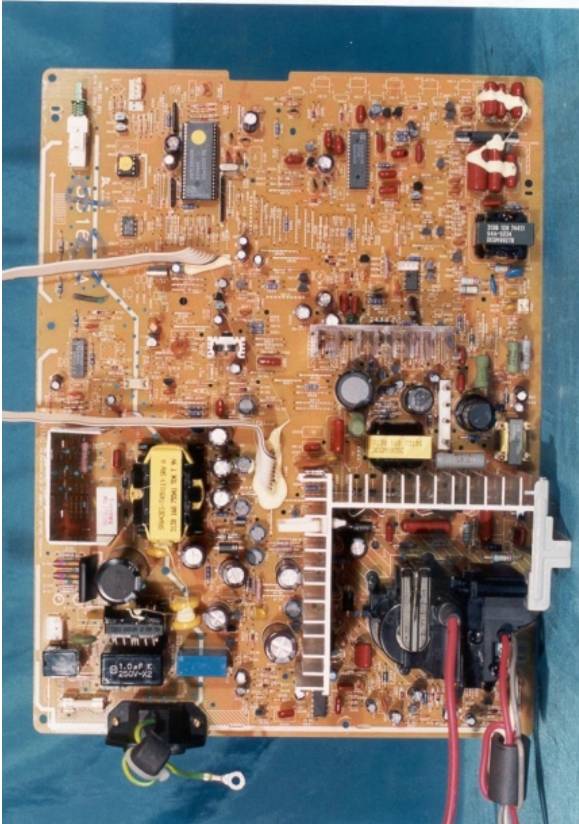
PCB Layout
