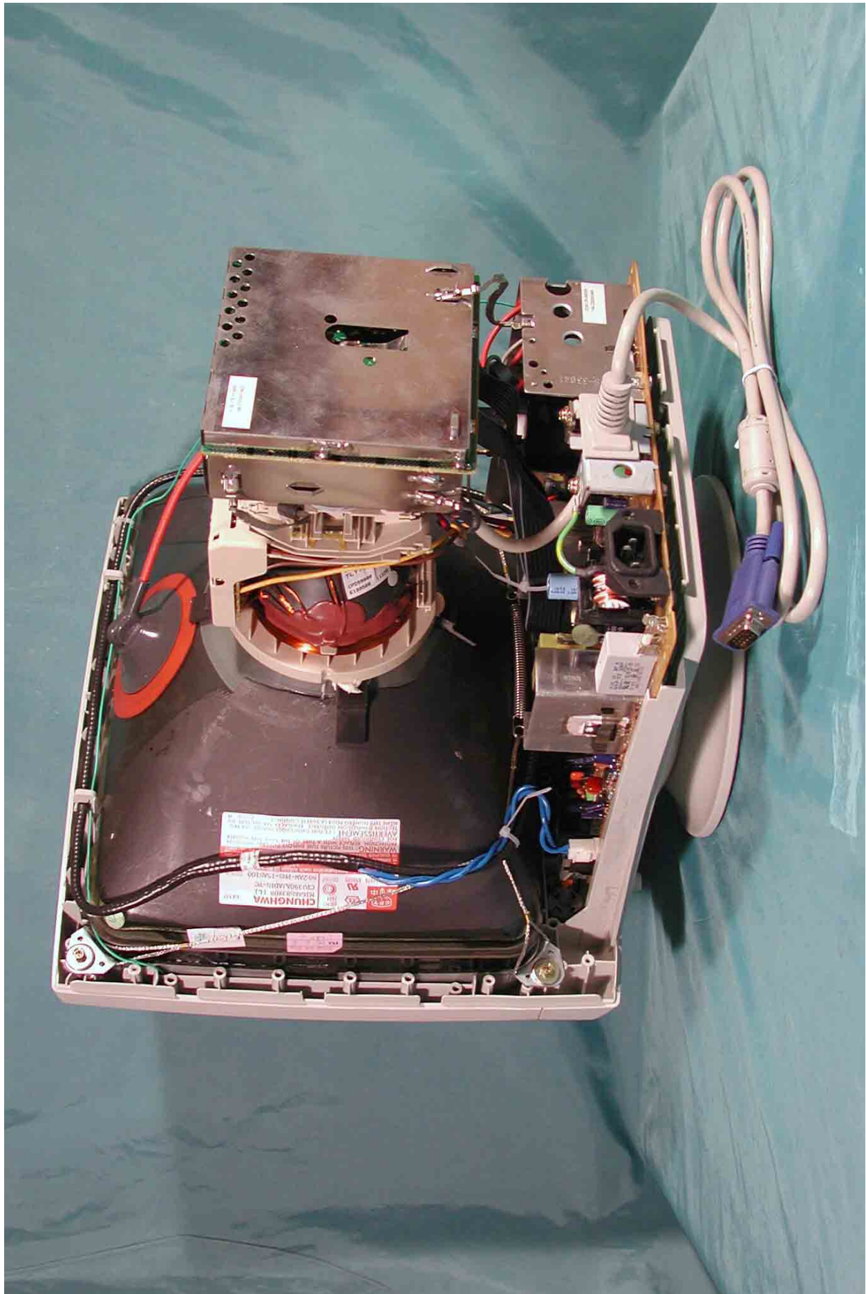
Side View Without Back Cover (CPT CRT)
