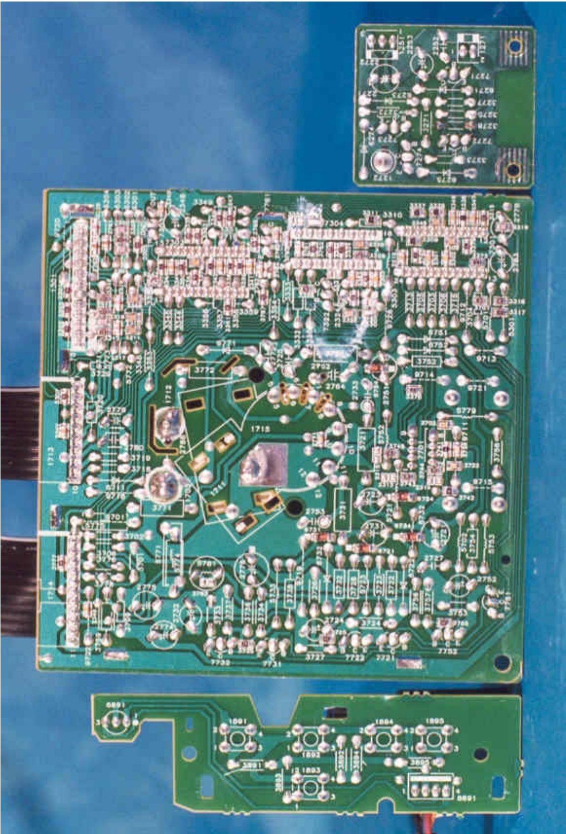
PCB Layout
