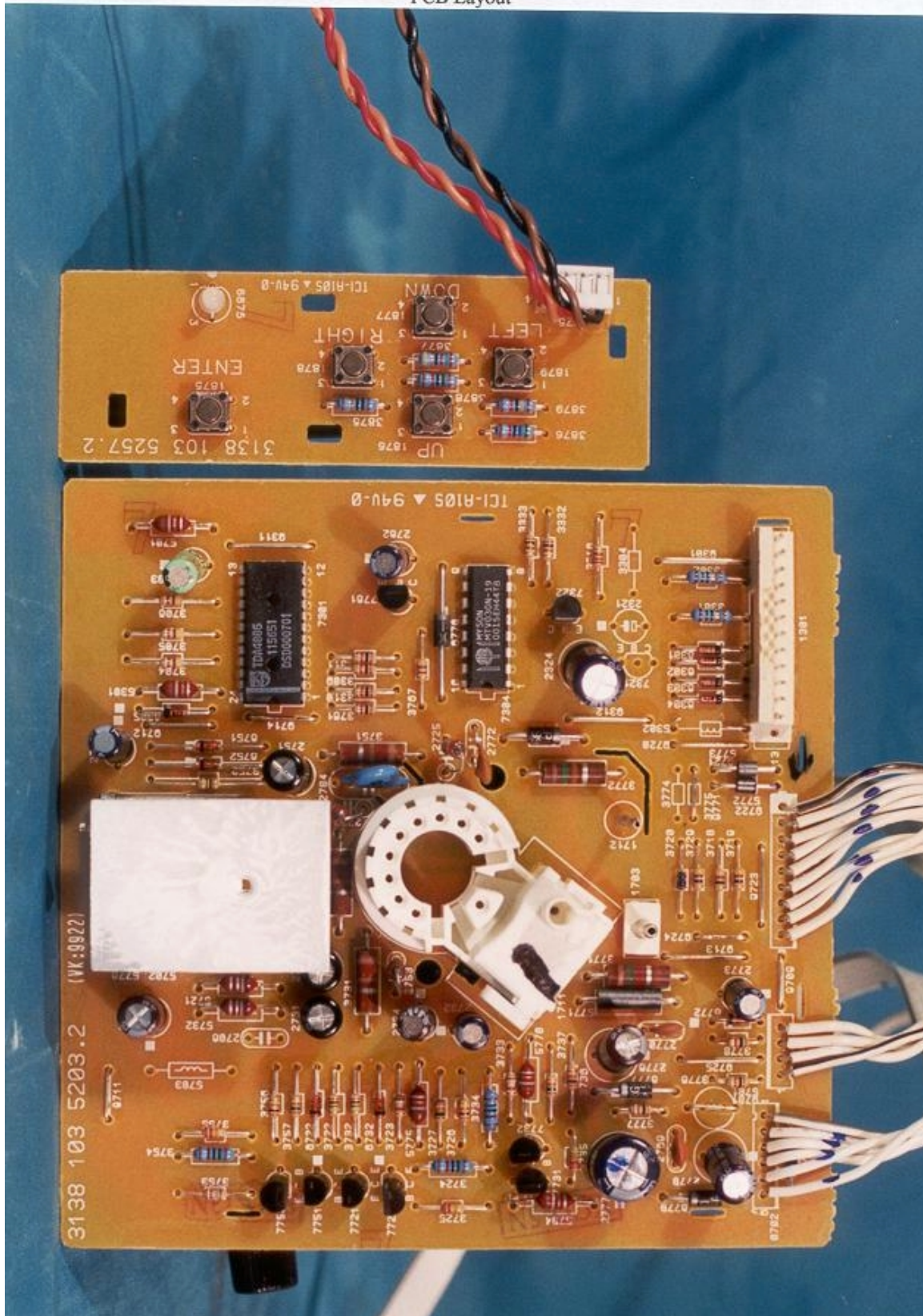
PCB Layout
