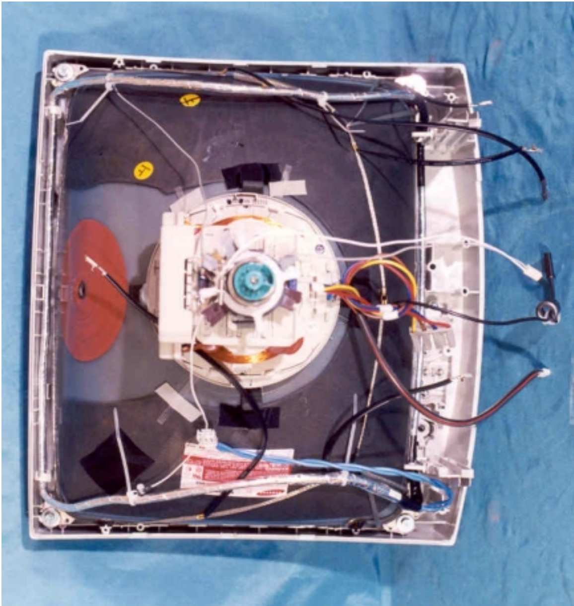
CRT Assembly
