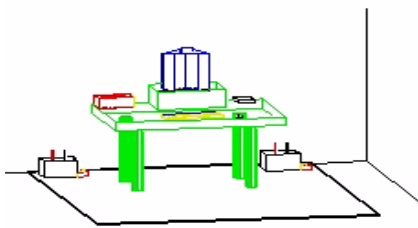
Figure 3. Line Conducted
