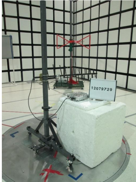
RADIATED FRONT UHF LOG PERIODIC ANTENNA
