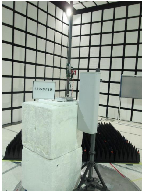
RADIATED FRONT UHF PANEL ANTENNA
