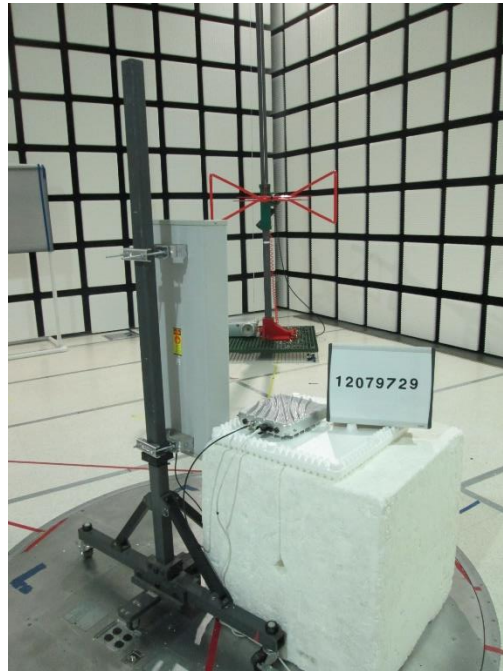
RADIATED FRONT UHF PANEL ANTENNA
