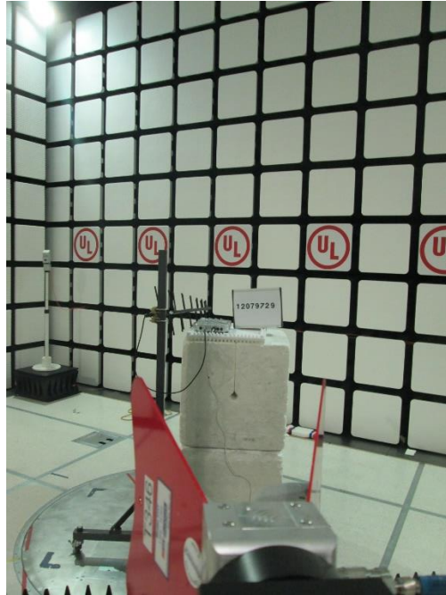
RADIATED FRONT UHF LOG PERIODIC ANTENNA
