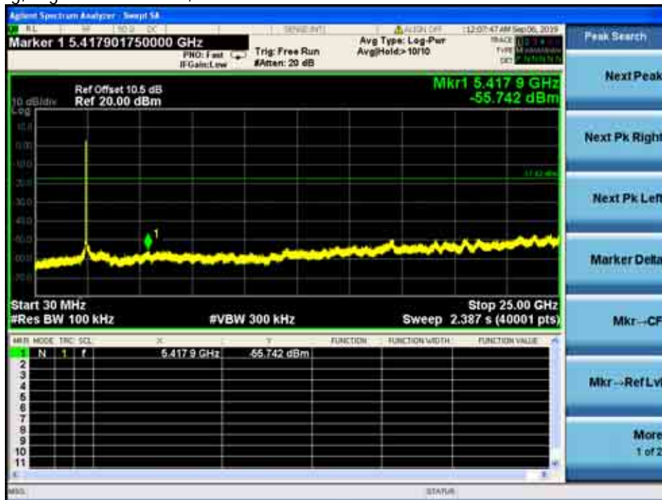
Ant.1_802.11g, Highest Channel-1, Plot B
