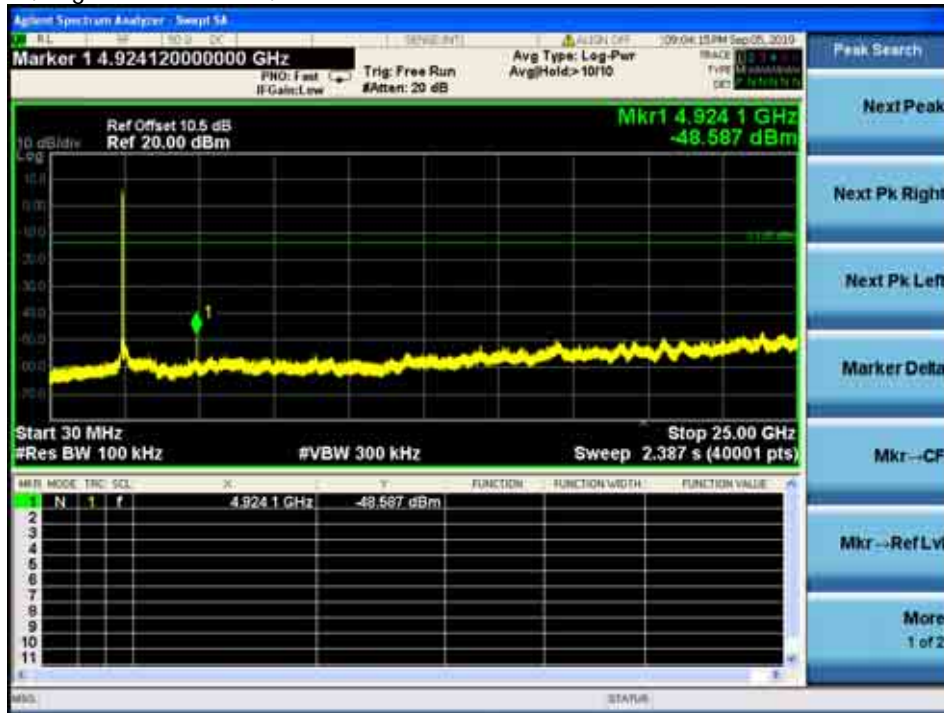
Ant.2_802.11b, Highest Channel-1, Plot B
