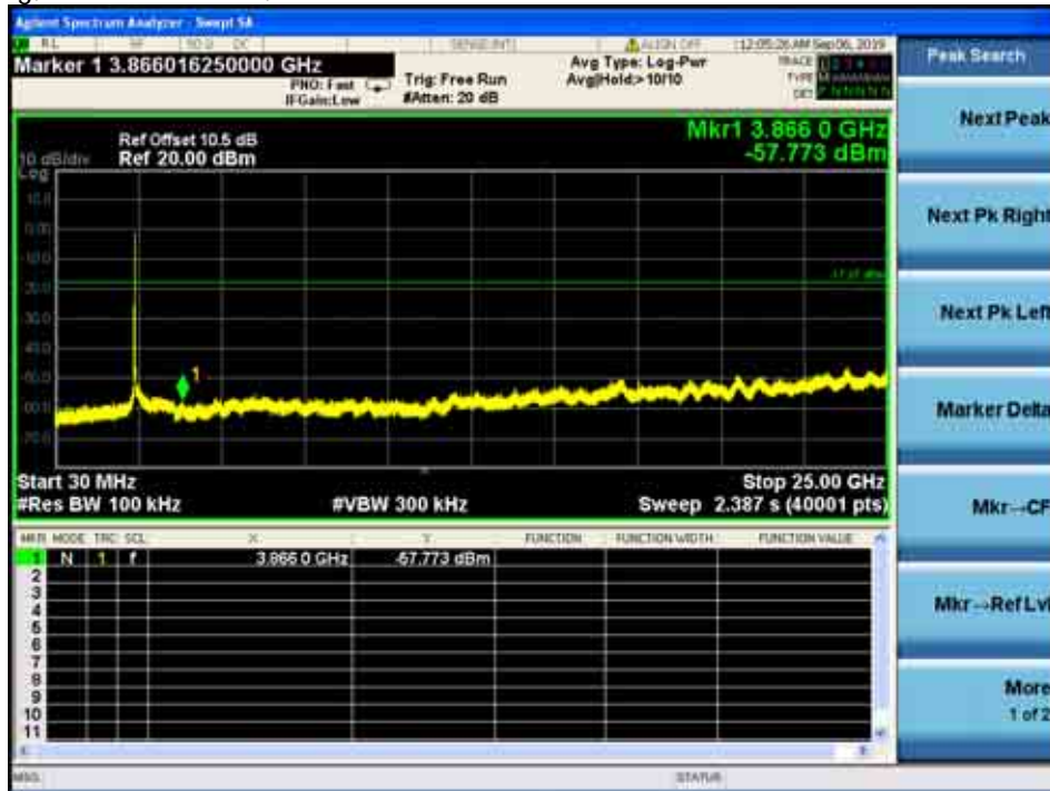
Ant.1_802.11g, Lowest Channel, Plot B
