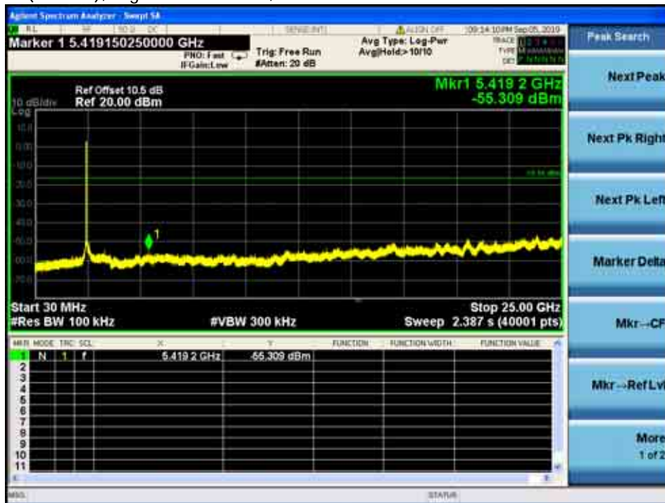
Ant.2_802.11n (20MHz), Highest Channel-2, Plot B
