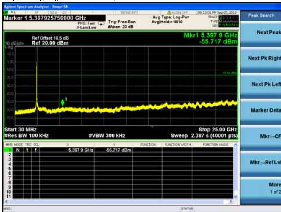
Ant.2_802.11n (20MHz), Highest Channel-3, Plot B
