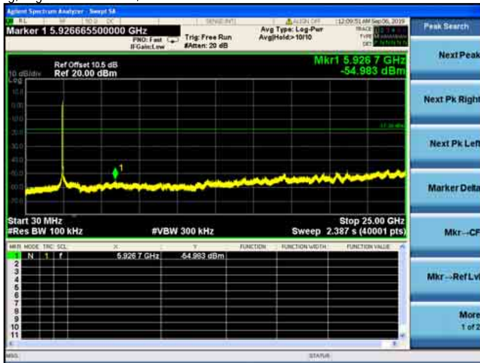
Ant.1_802.11g, Highest Channel-2, Plot B
