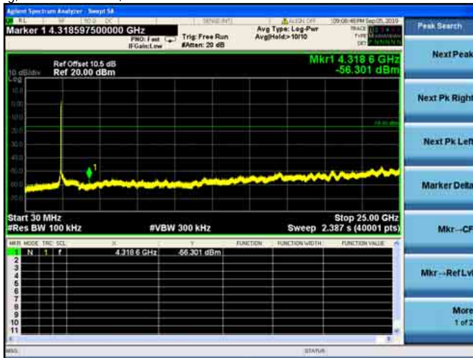
Ant.2_802.11g, Middle Channel, Plot B
