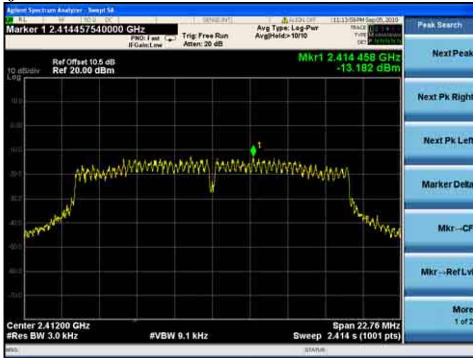
Ant.1_802.11g, Lowest channel
