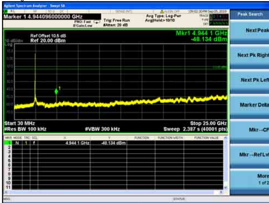
Ant.2_802.11b, Highest Channel-3, Plot B
