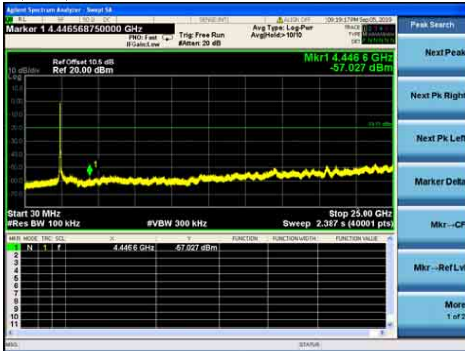
Ant.2_802.11n (40MHz), Middle Channel, Plot B
