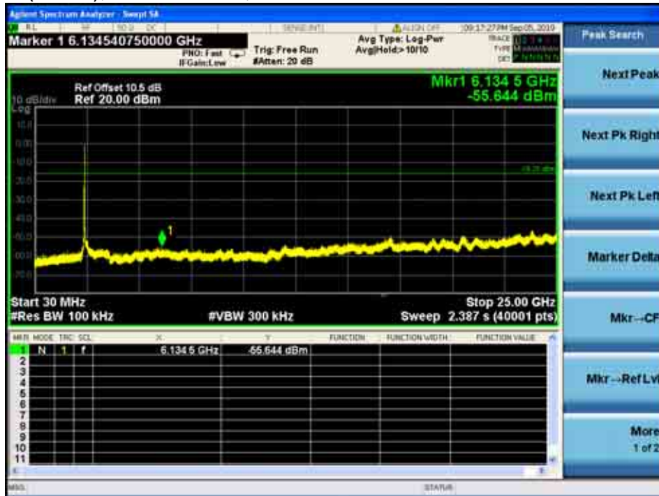
Ant.2_802.11n (20MHz), Lowest Channel, Plot B
