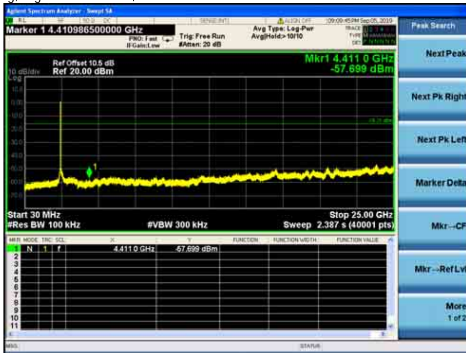
Ant.2_802.11g, Highest Channel-1, Plot B
