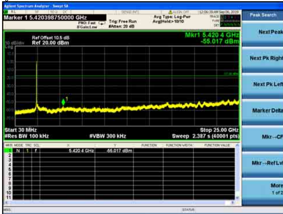
Ant.1_802.11g, Middle Channel, Plot B
