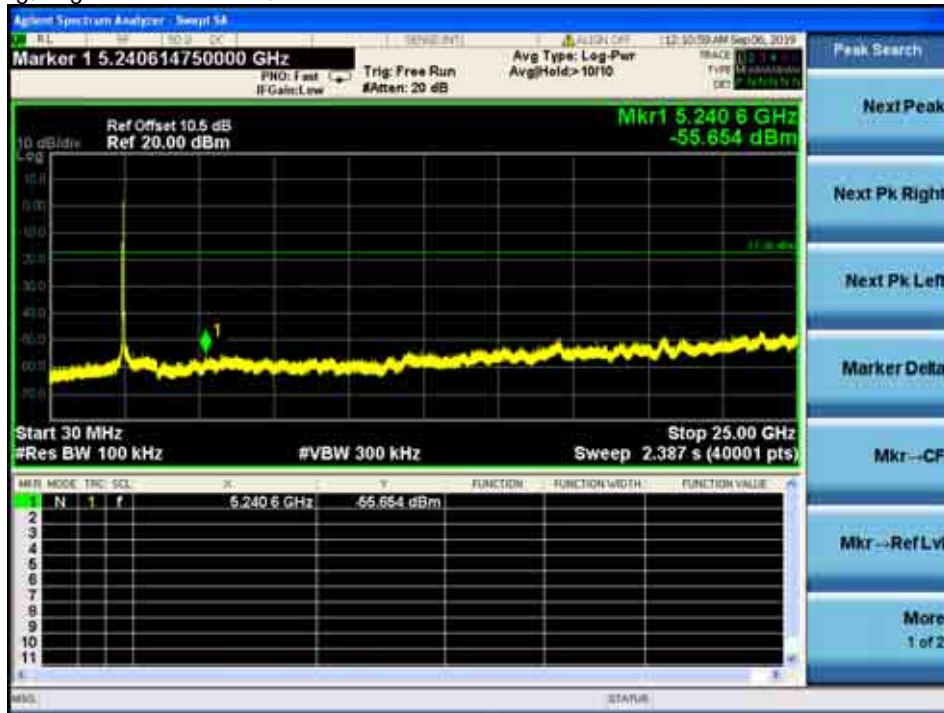
Ant.1_802.11g, Highest Channel-3, Plot B
