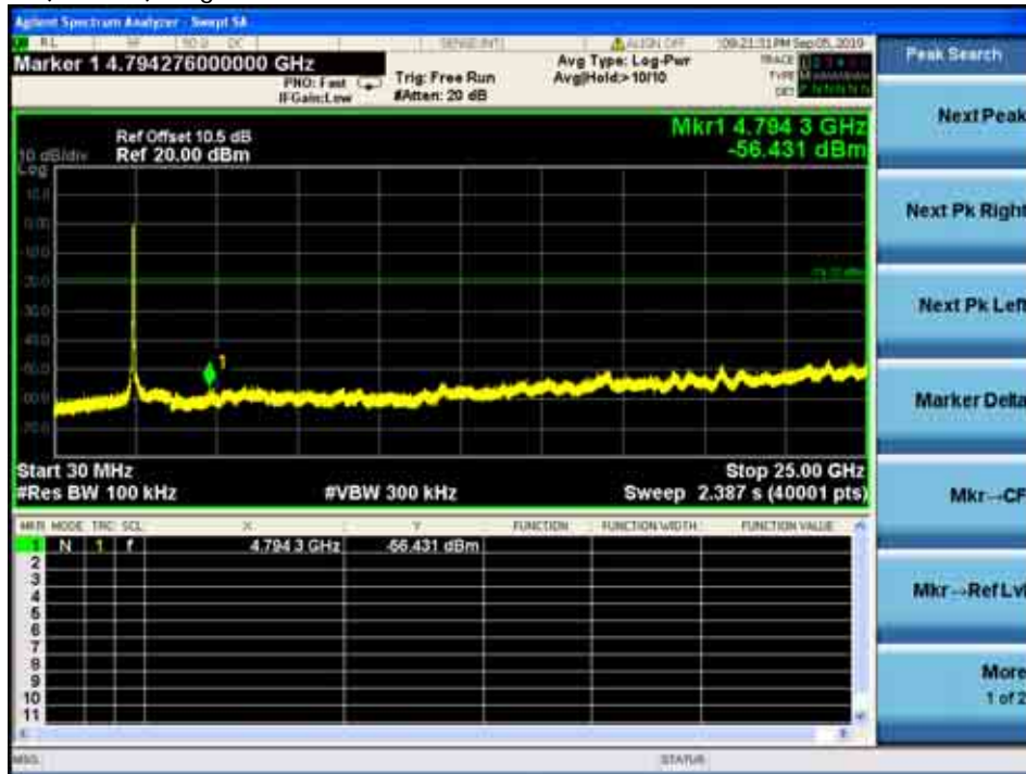
Ant.2_802.11n (40MHz), Highest Channel-1, Plot B
