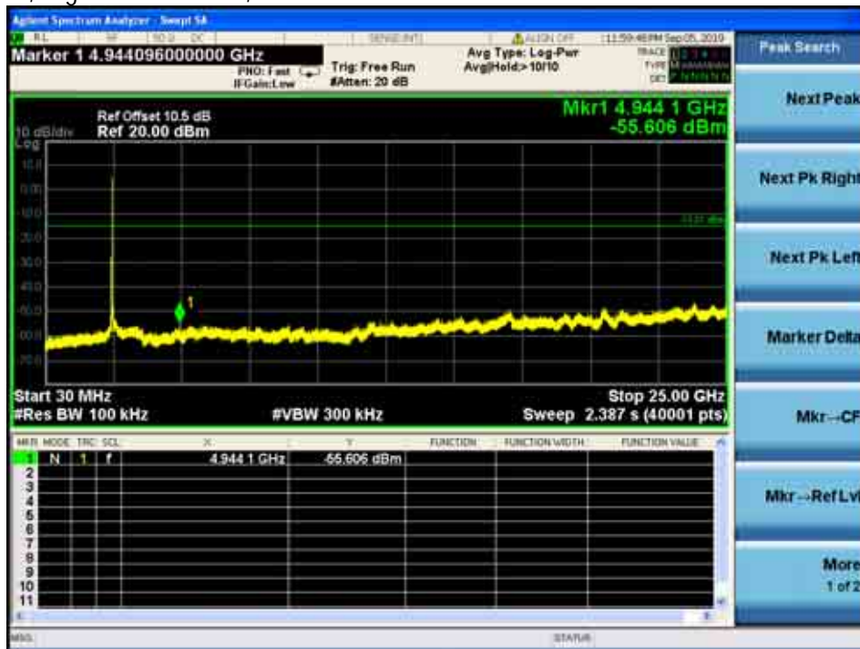
Ant.1_802.11b, Highest Channel-3, Plot B
