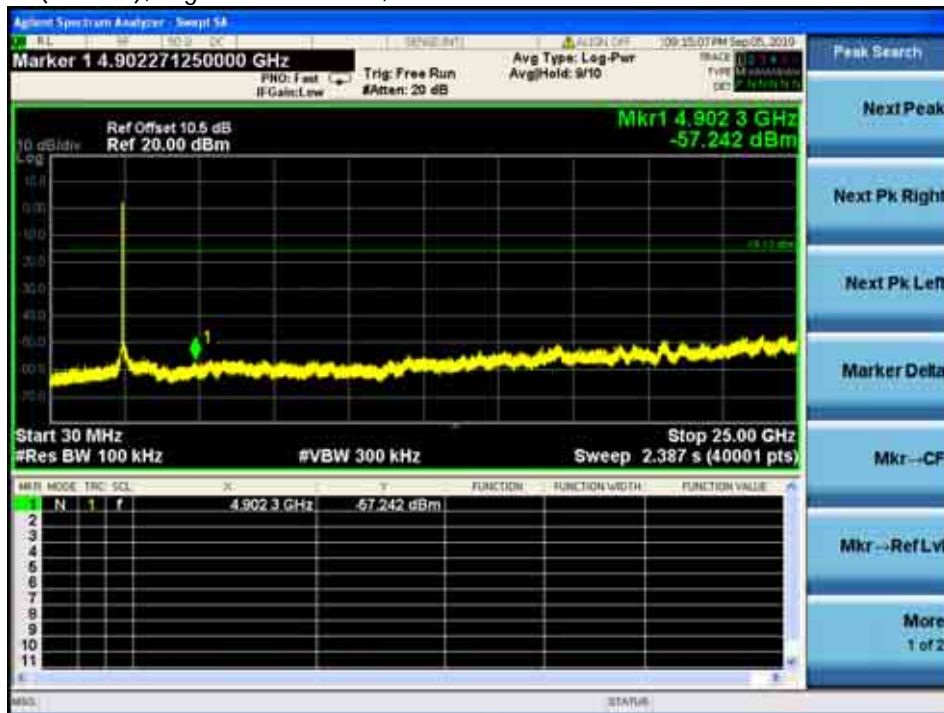
Ant.2_802.11n (20MHz), Highest Channel-1, Plot B
