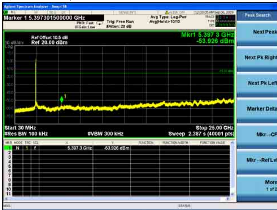
Ant.1_802.11b, Middle Channel, Plot B
