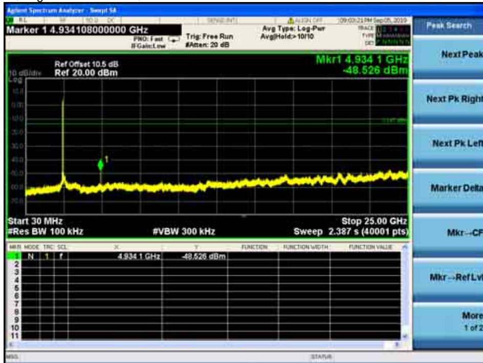
Ant.2_802.11b, Highest Channel-2, Plot B
