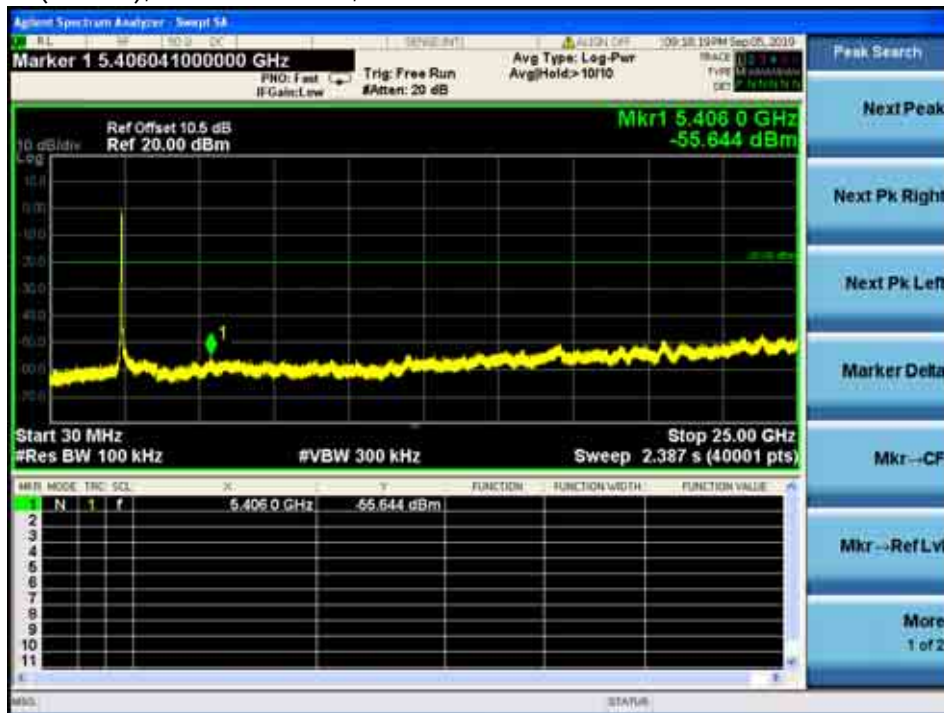
Ant.2_802.11n (40MHz), Lowest Channel, Plot B
