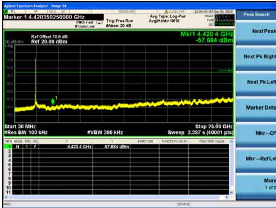
Ant.1_802.11b, Lowest Channel, Plot B
