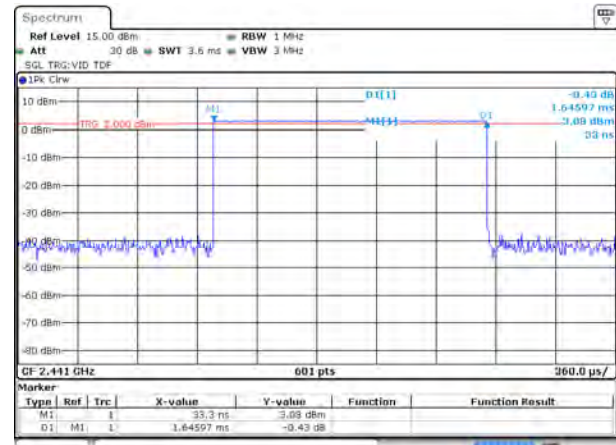
GFSK DH3
