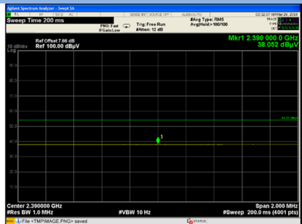
8-DPSK LOW CHANNEL , AVERAGE
