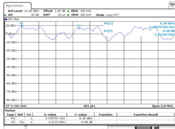
8-DPSK
