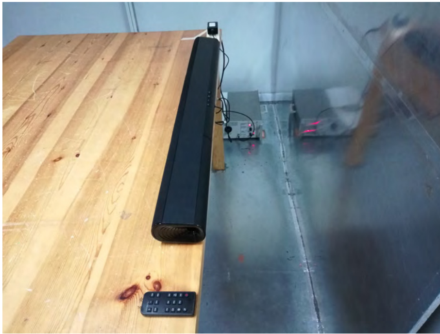
Conducted Emission Test (GT-WWLA13000180-302)
