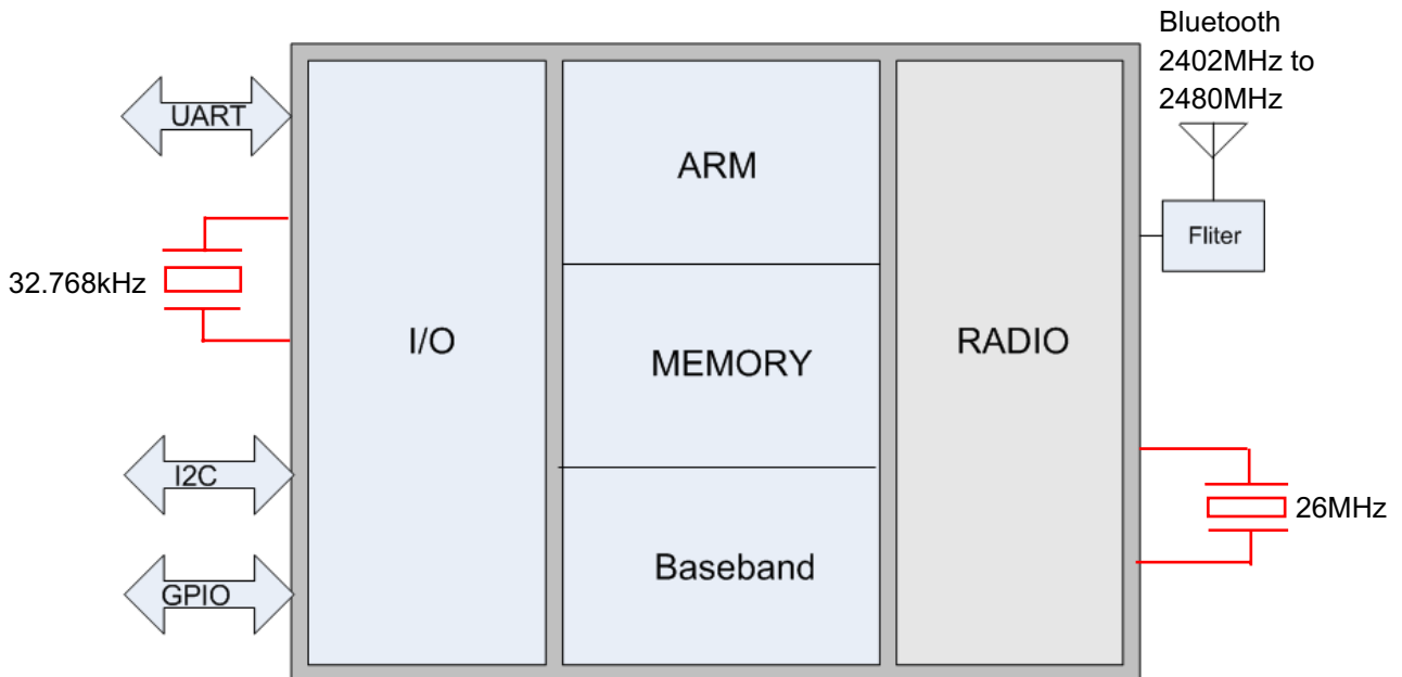
Figure3-1. RDA5876 Bluetooth Block Diagram
