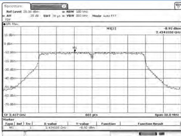
802.11n-20 MHz MIDDLE CHANNEL CARRIER LEVEL
