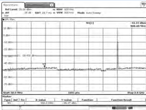
802.11n-20 MHz LOW CHANNEL, SPURIOUS 30 MHz ~ 3 GHz
