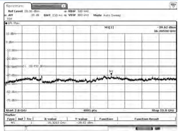
802.11n-20 MHz LOW CHANNEL, SPURIOUS 2 GHz ~ 25 GHz
