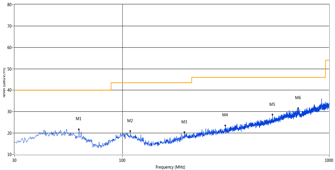
30 MHz to 1 GHz, ANT V
