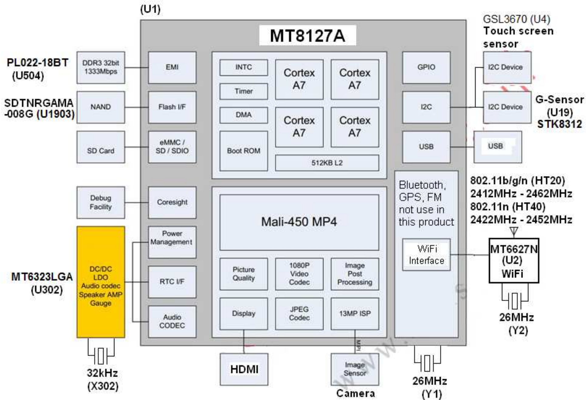
Block Diagram
