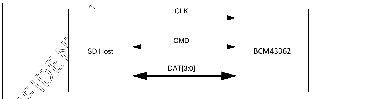
Figure 7: Signal Connections to SDIO Host (SD 4-Bit Mode)
