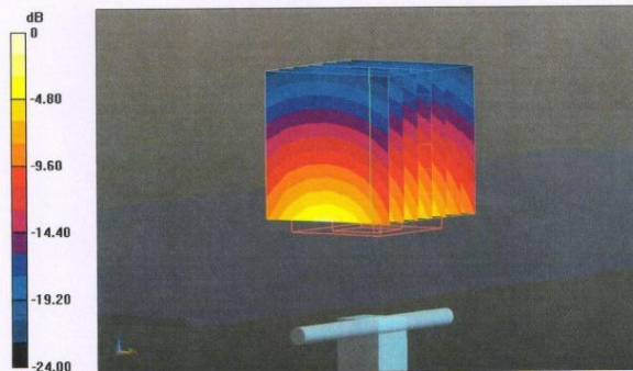
0 dB = 18.2 W/kg = 12.60 dBW/kg
