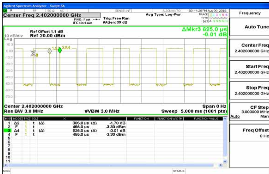
Duty Cycle_BLE_1M_LowCH00-2402
