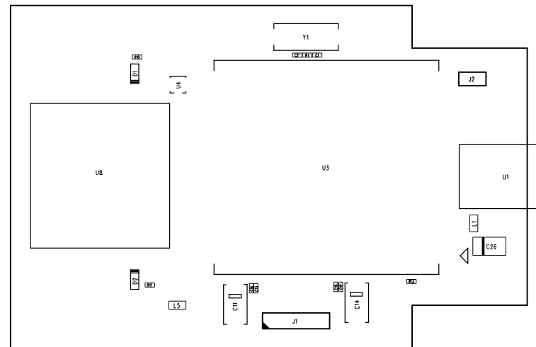
Assembly Drawing Top
