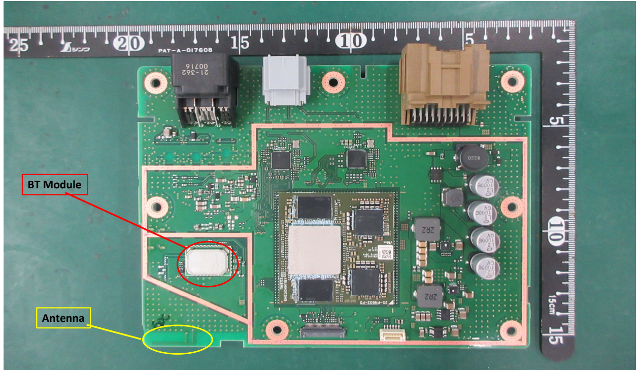
PCB Bottom view
