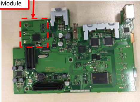
PANEL I.MX surface
