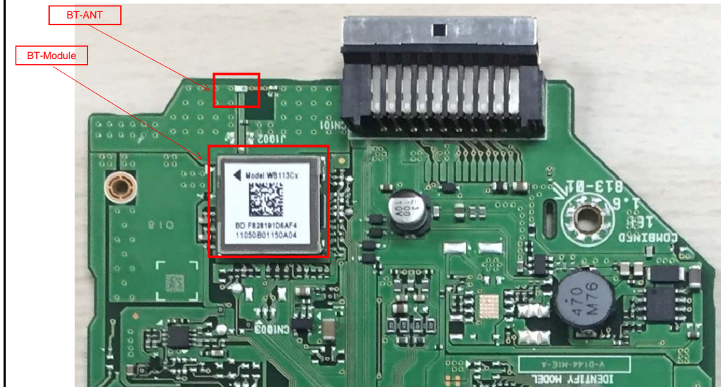
Position of BT ANT and the BT module
