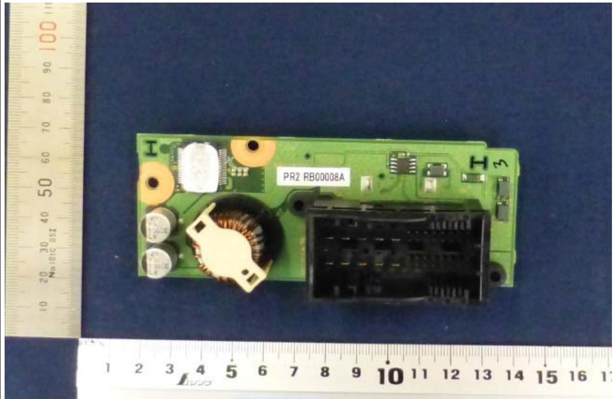
REAR PCB Top view
