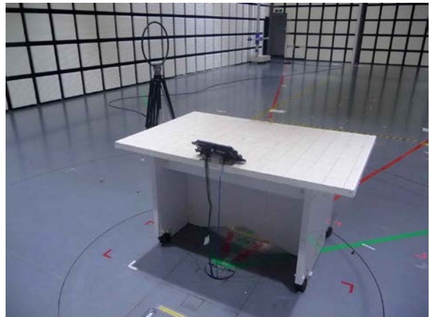
Antenna: Vertical
