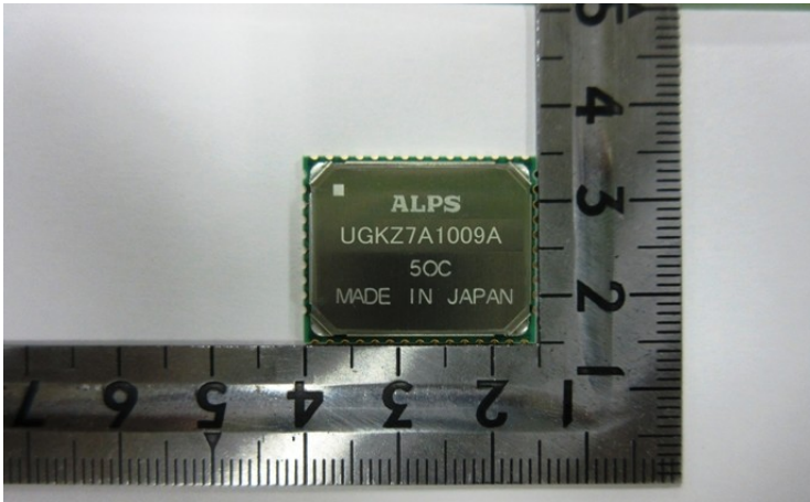
UGKZ7A1 with shield cover
