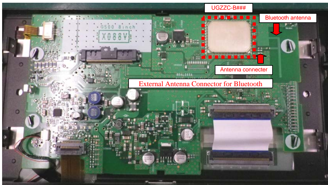
Fig 2. Reverse View of Display unit that installed Bluetooth Transmitter “UGZC-B###”
