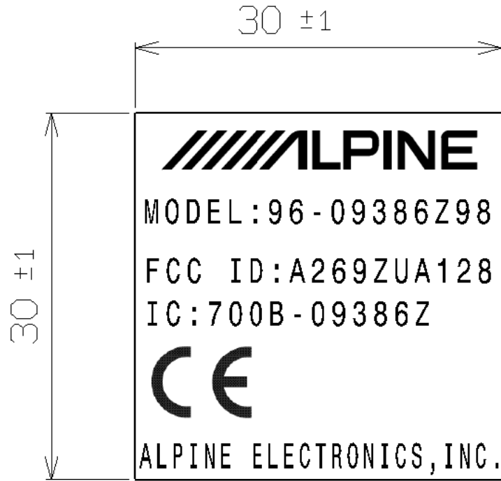
Label Drawing
