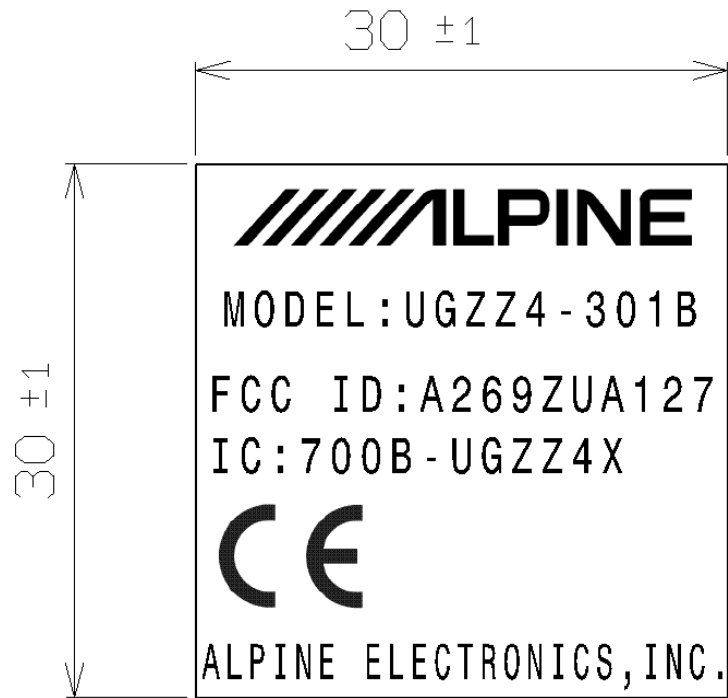
Label Drawing
