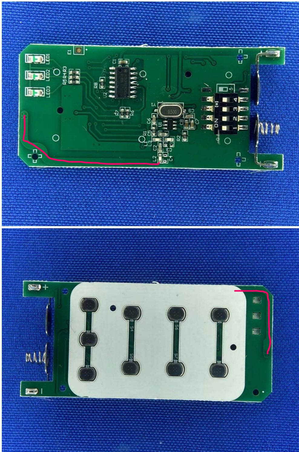
Antenna Gain: PCB antenna with maximum gain 0 dBi
