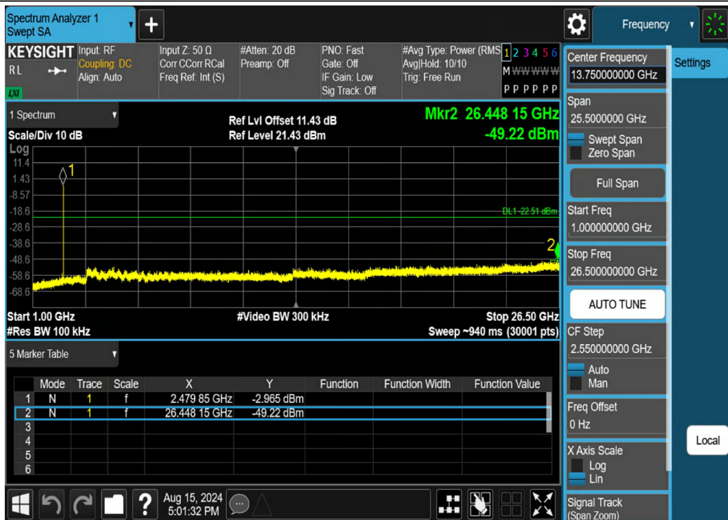
BLE_2M-Ant1-2480-1000~26500-PASS
