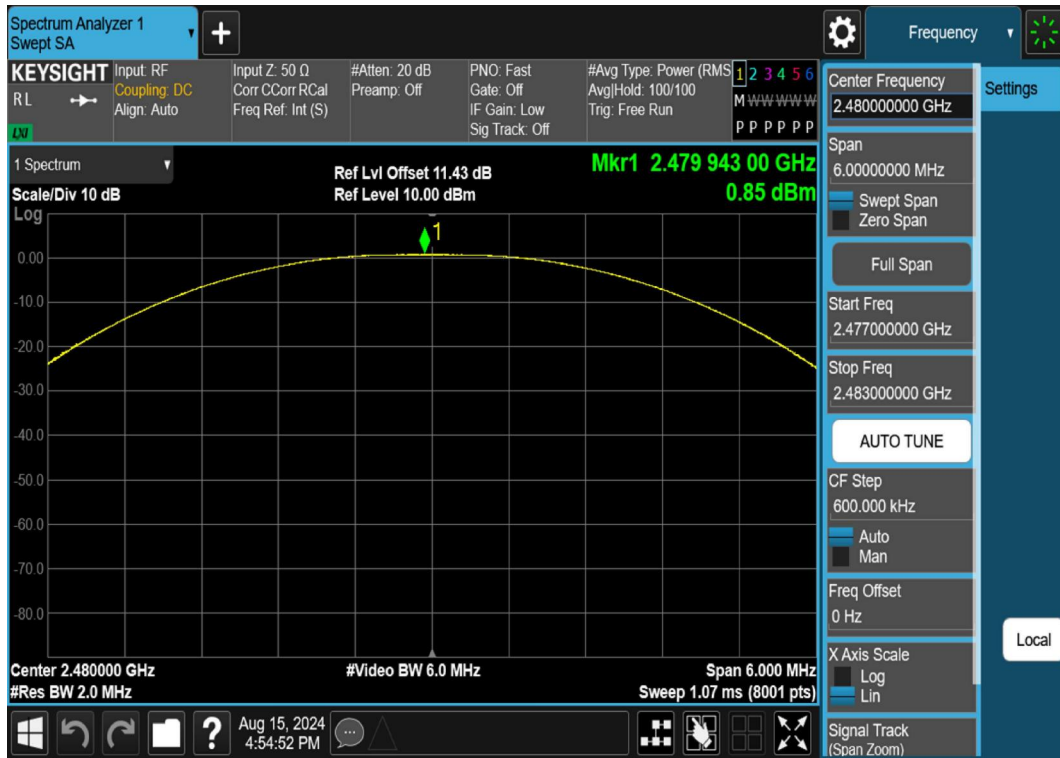
BLE_1M-Ant1-2480-PASS
