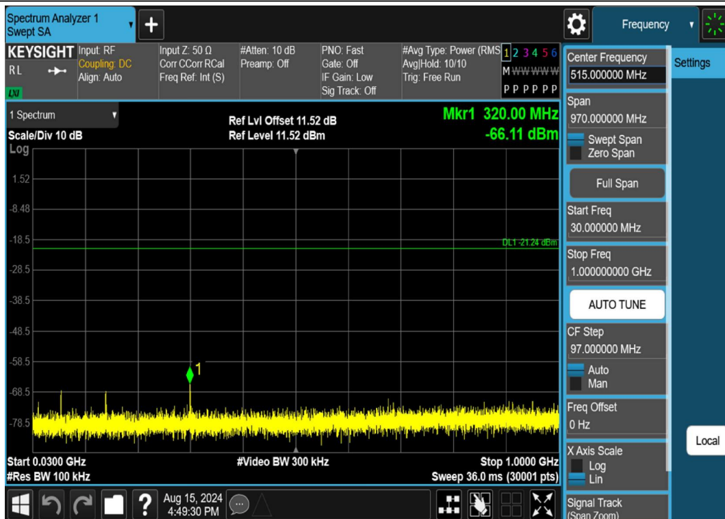
BLE_1M-Ant1-2402-30~1000-PASS
