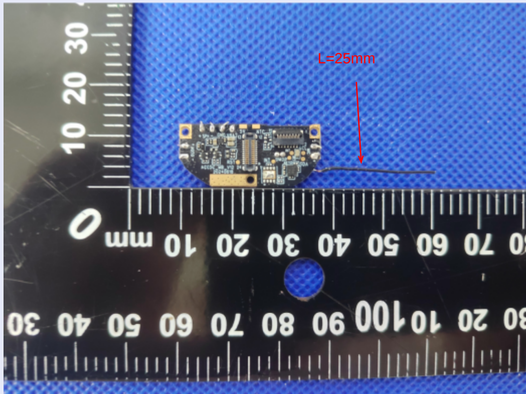
Antenna Photo & Length (mm)
