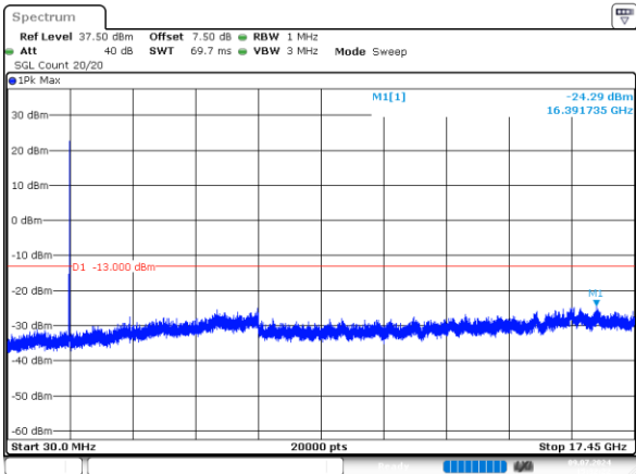
10MHz_Middle_QPSK_1@0 -24.29dBm
