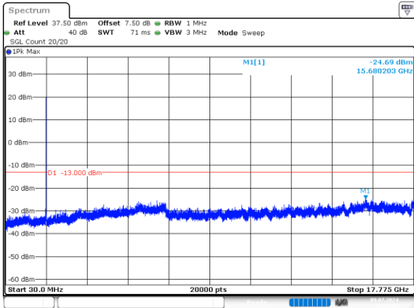
5MHz_High_QPSK_25@0 -24.69dBm
