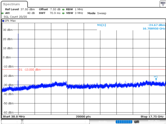
10MHz_High_QPSK_1@0 -24.67dBm
