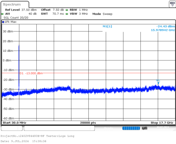
20MHz_High_QPSK_100@0 -24.43dBm
