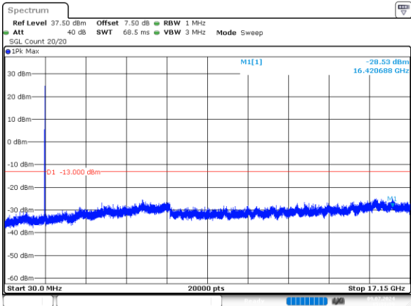
10MHz_Low_QPSK_1@0 -28.53dBm
