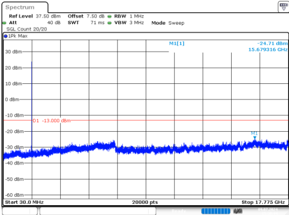
5MHz_High_QPSK_1@0 -24.71dBm
