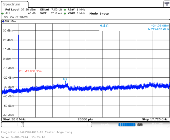
15MHz_High_QPSK_1@0 -24.98dBm
