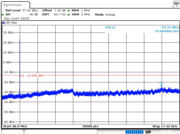
5MHz_Middle_QPSK_1@0 -24.31dBm
