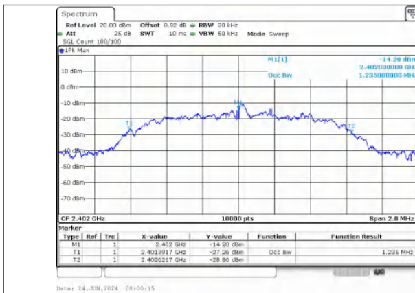
8DPSK_3-DH5_Channel 0
