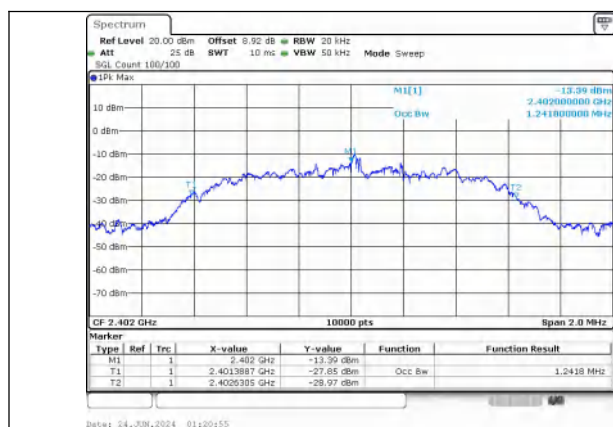
8DPSK_3-DH5_Channel 0
