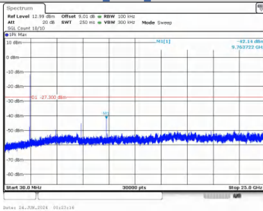
30.0 MHz - 25000.0 MHz 8DPSK_3-DH5_Channel 30
