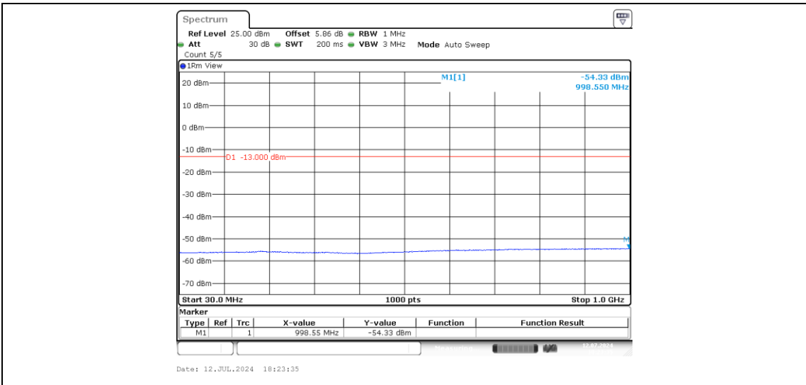
Band2-10MHz-QPSK-18900-1-0-Low-30-1000--54.33-PASS
