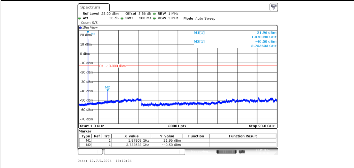
Band2-5MHz-QPSK-18900-1-0-Low-1000-20000--40.5-PASS
