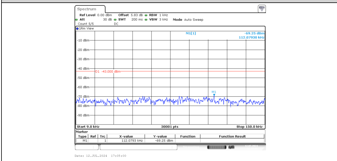
Band2-15MHz-QPSK-19125-1-0-High-0.009-0.15--69.25-PASS
