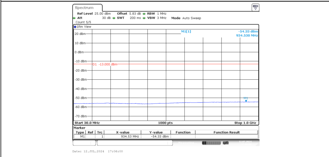
Band2-15MHz-16QAM-19125-1-0-High-30-1000--54.33-PASS
