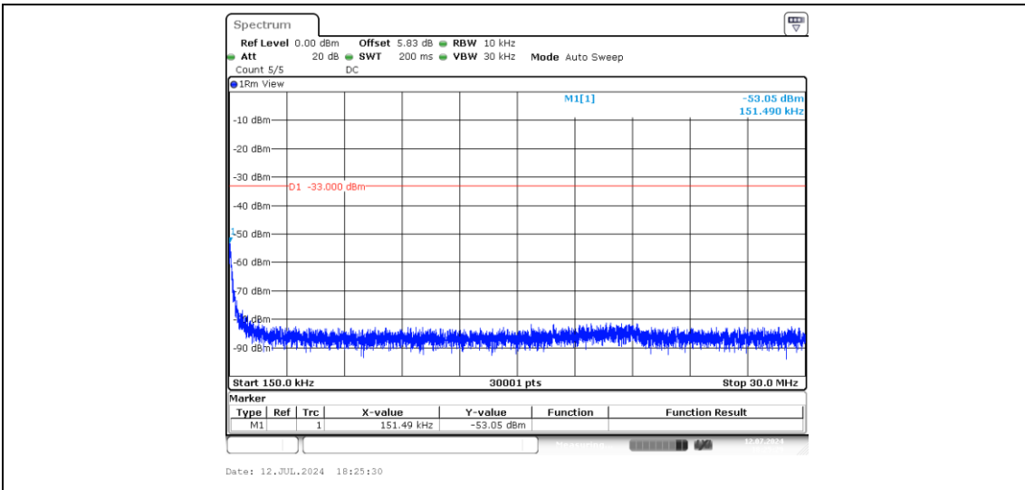
Band2-10MHz-16QAM-19150-1-0-High-0.15-30--53.05-PASS
