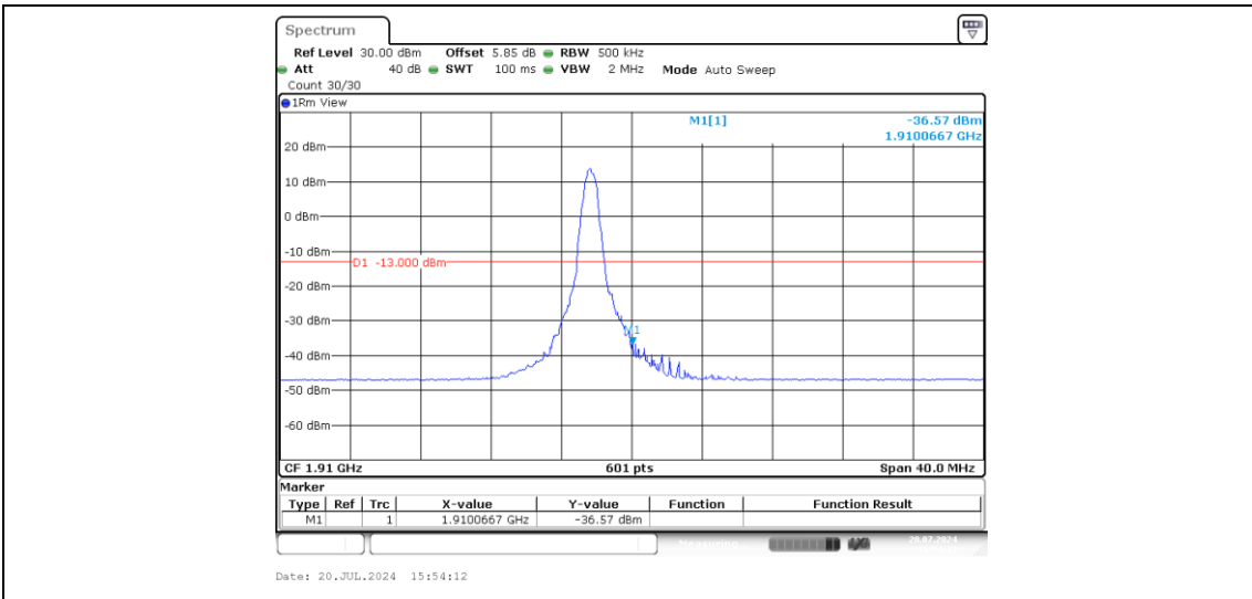
Band2-20MHz-16QAM-19100-1-0-High--36.57-PASS
