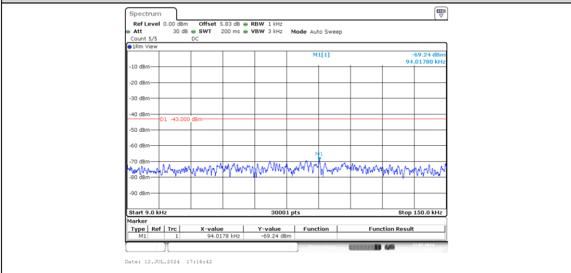
Band2-20MHz-QPSK-19100-1-0-High-0.009-0.15--69.24-PASS
