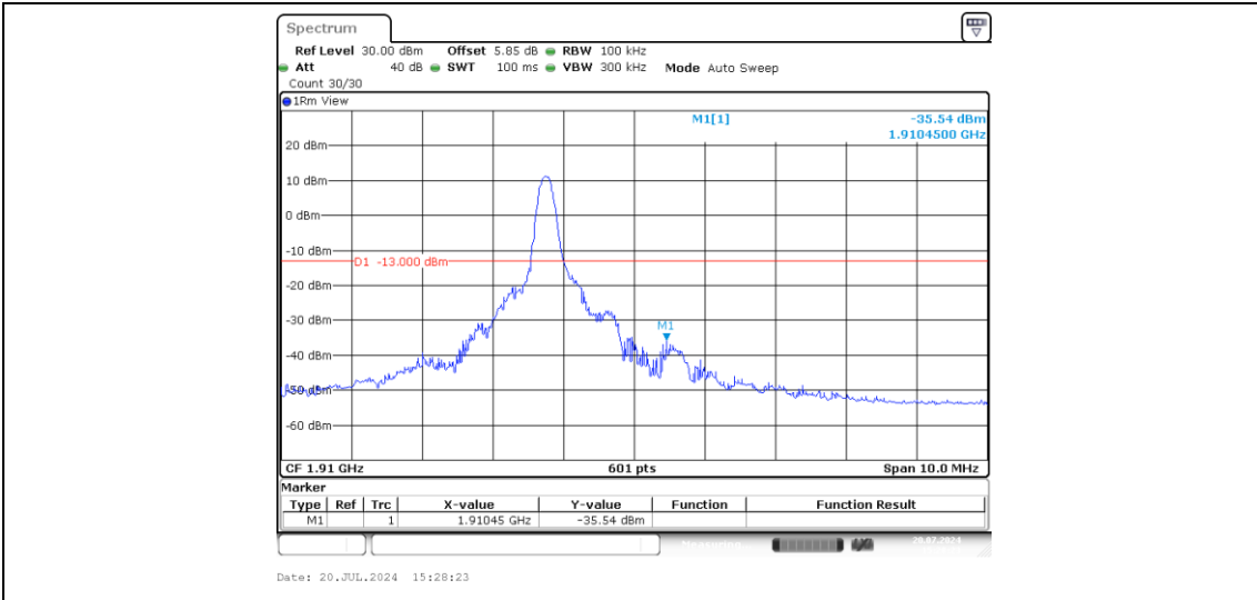
Band2-5MHz-16QAM-19175-1-0-High--35.54-PASS
