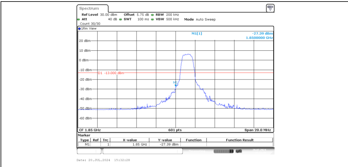
Band2-10MHz-QPSK-18650-6-0-Low--27.39-PASS
