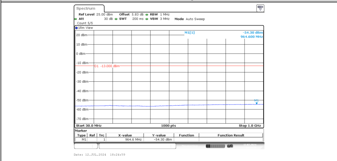
Band2-10MHz-QPSK-19150-1-0-High-30-1000--54.3-PASS
