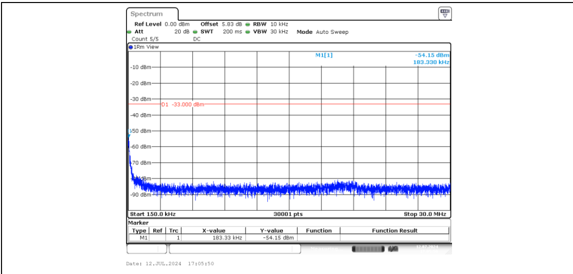
Band2-15MHz-16QAM-19125-1-0-High-0.15-30--54.15-PASS
