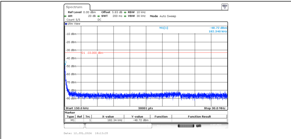
Band2-5MHz-QPSK-19175-1-0-High-0.15-30--48.72-PASS
