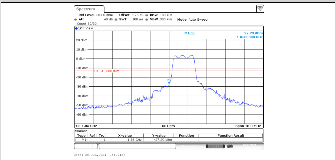
Band2-5MHz-16QAM-18625-6-0-Low--27.29-PASS
