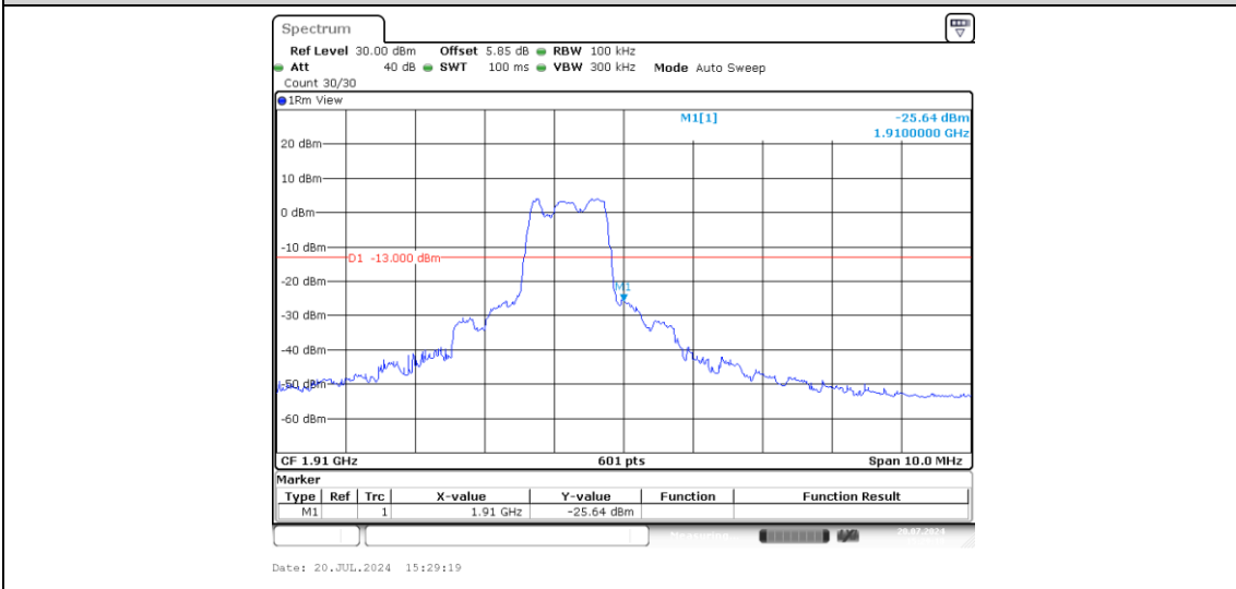
Band2-5MHz-16QAM-19175-6-0-High--25.64-PASS
