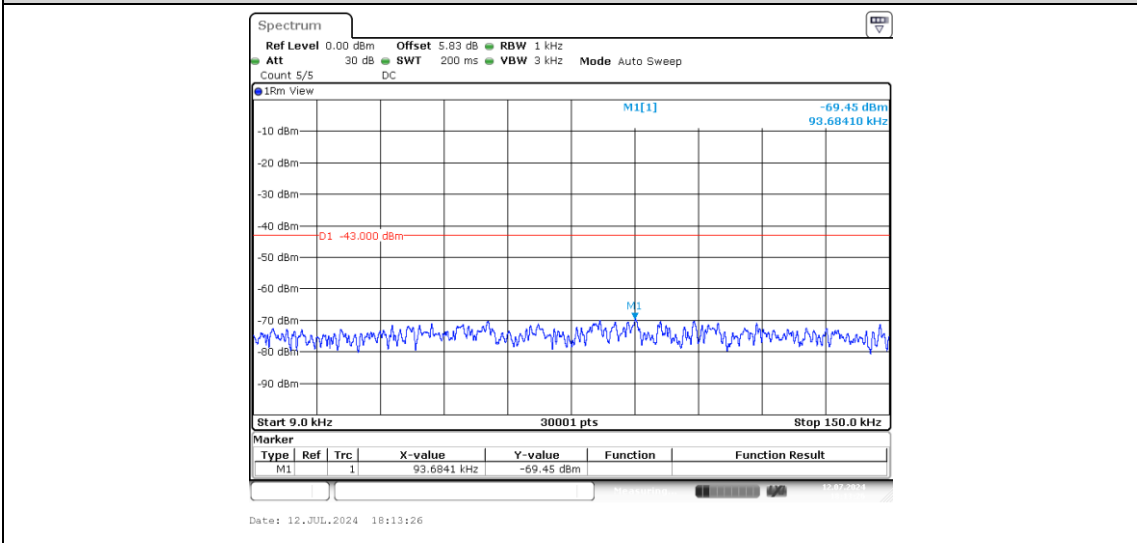
Band2-5MHz-QPSK-19175-1-0-High-0.009-0.15--69.45-PASS
