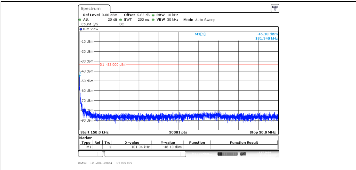
Band2-15MHz-QPSK-19125-1-0-High-0.15-30--46.18-PASS
