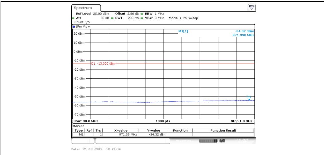
Band2-10MHz-16QAM-18900-1-0-Low-30-1000--54.32-PASS
