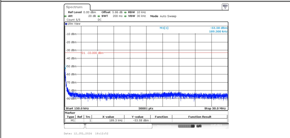
Band2-5MHz-16QAM-18900-1-0-Low-0.15-30--53.58-PASS
