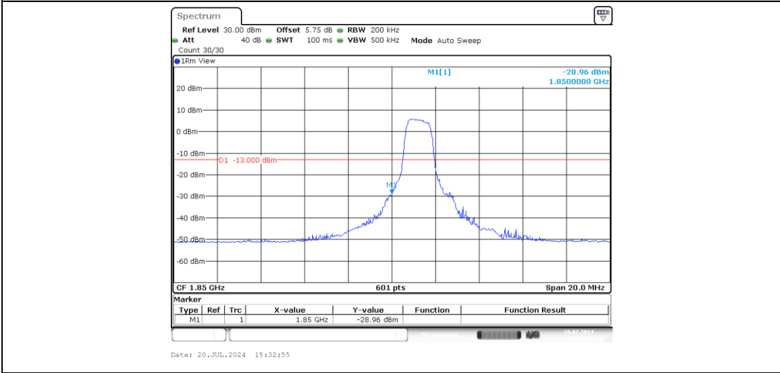
Band2-10MHz-16QAM-18650-6-0-Low--28.96-PASS
