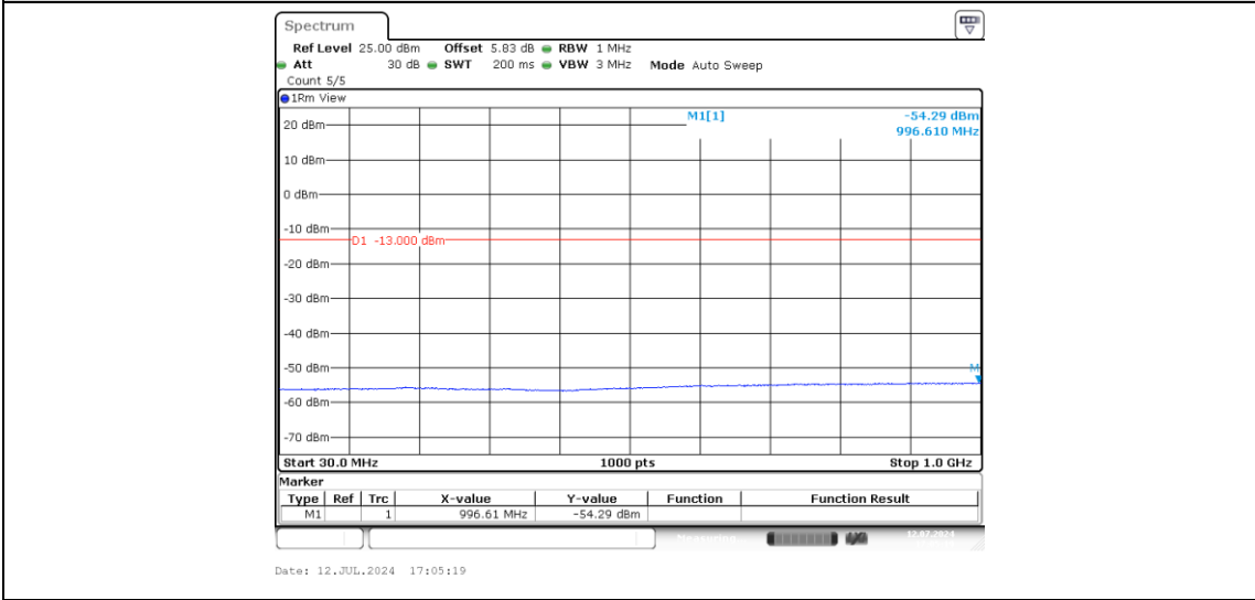
Band2-15MHz-QPSK-19125-1-0-High-30-1000--54.29-PASS
