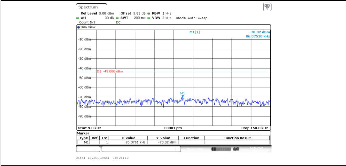
Band2-10MHz-QPSK-19150-1-0-High-0.009-0.15--70.32-PASS
