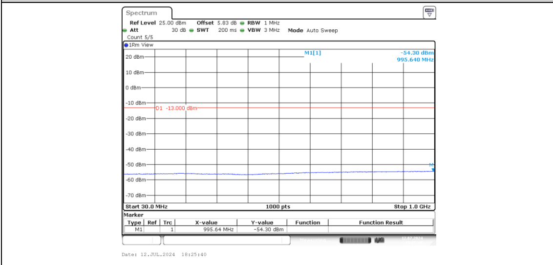
Band2-10MHz-16QAM-19150-1-0-High-30-1000--54.3-PASS
