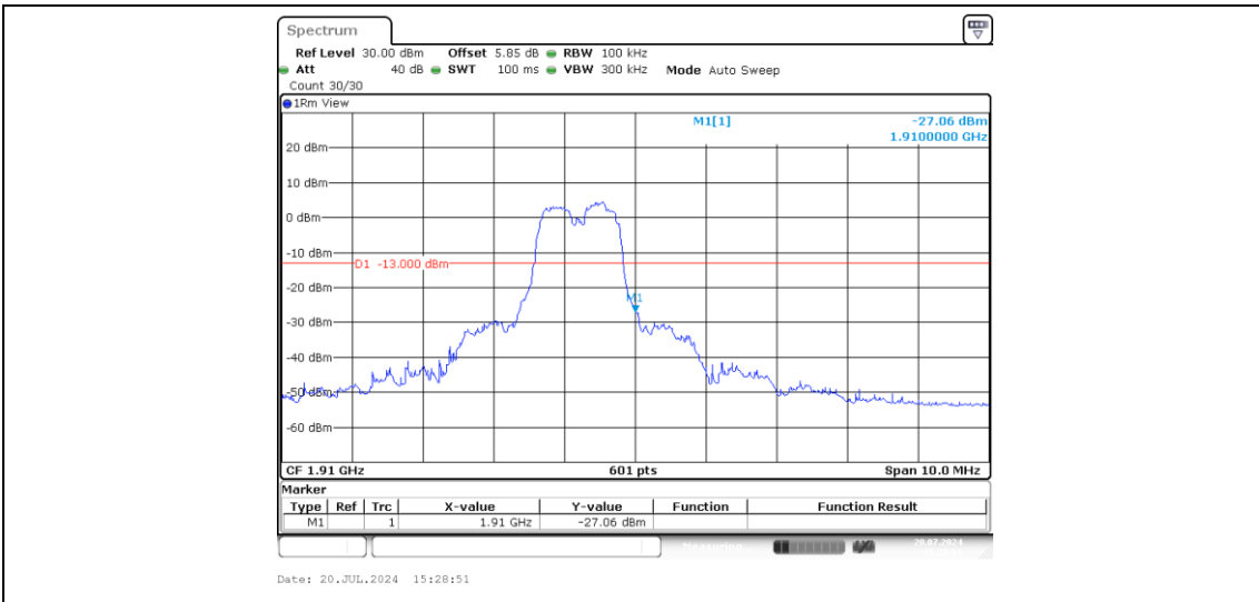
Band2-5MHz-QPSK-19175-6-0-High--27.06-PASS
