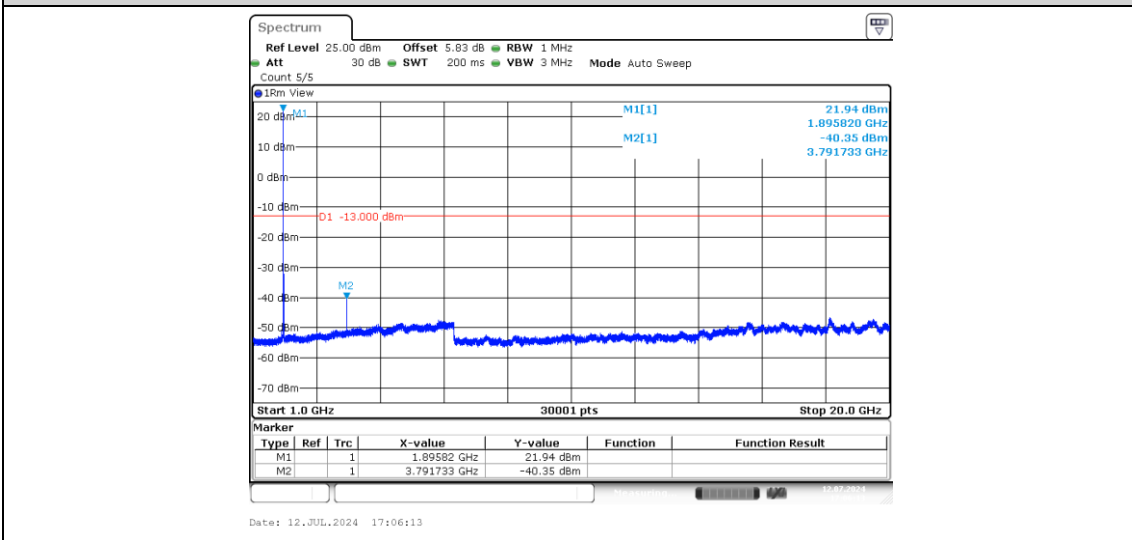
Band2-15MHz-16QAM-19125-1-0-High-1000-20000--40.35-PASS
