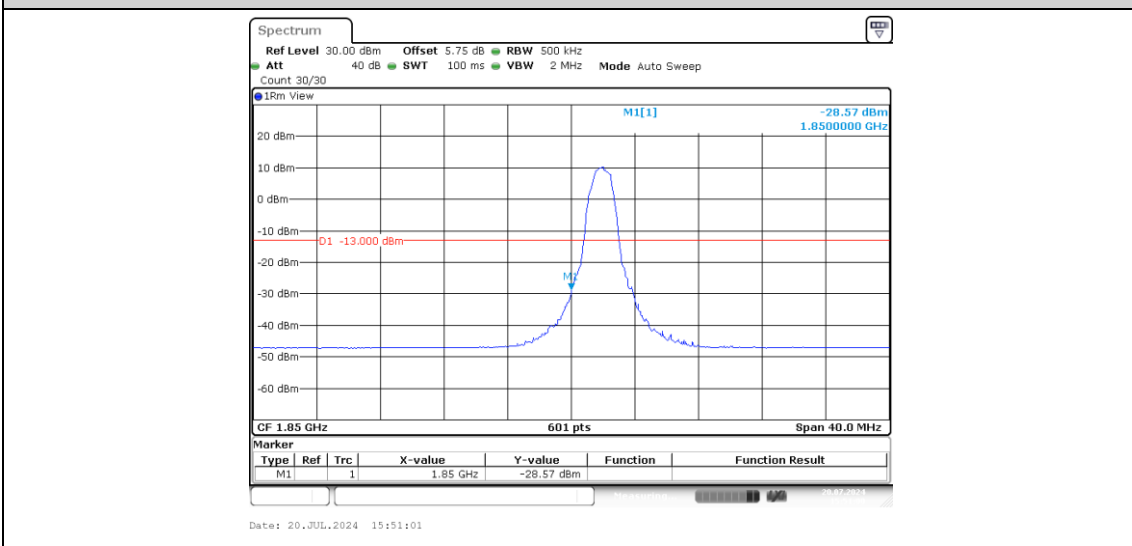
Band2-20MHz-16QAM-18700-6-0-Low--28.57-PASS
