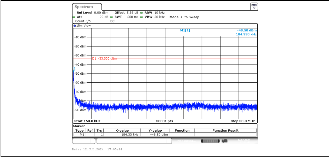
Band2-15MHz-QPSK-18900-1-0-Low-0.15-30--48.5-PASS
