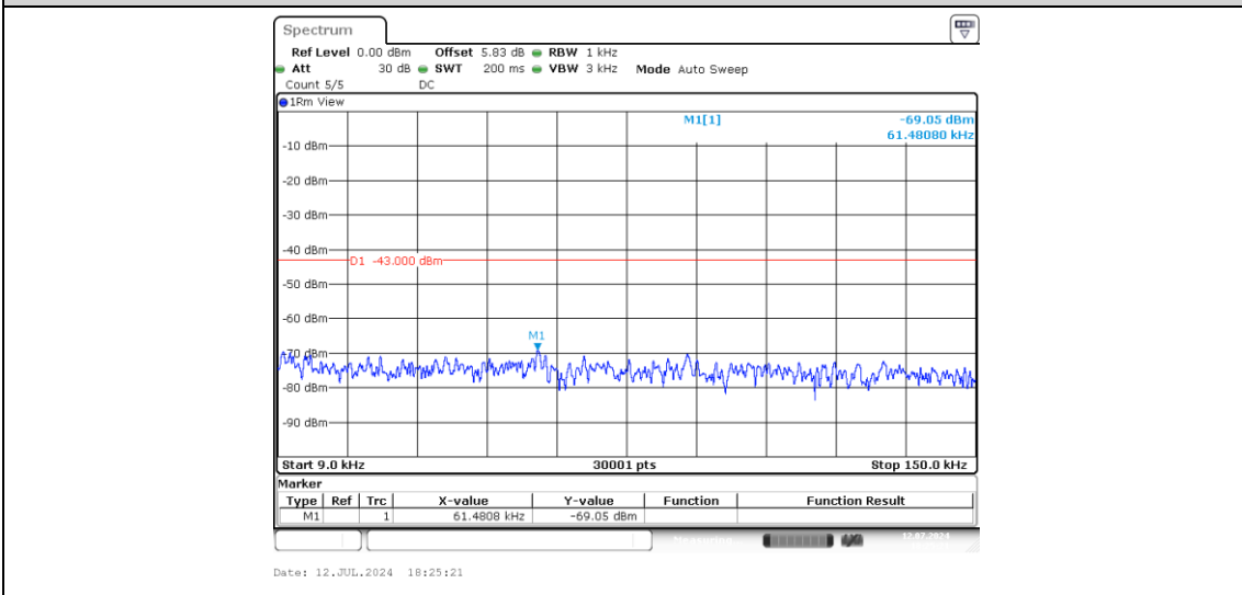
Band2-10MHz-16QAM-19150-1-0-High-0.009-0.15--69.05-PASS
