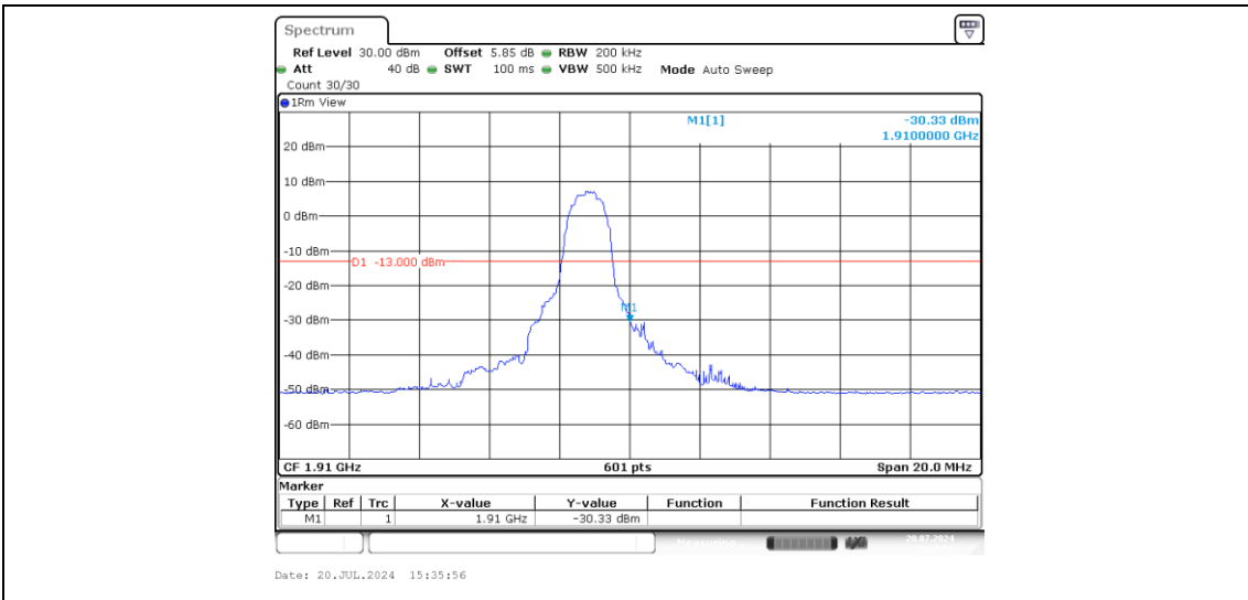
Band2-10MHz-16QAM-19150-6-0-High--30.33-PASS
