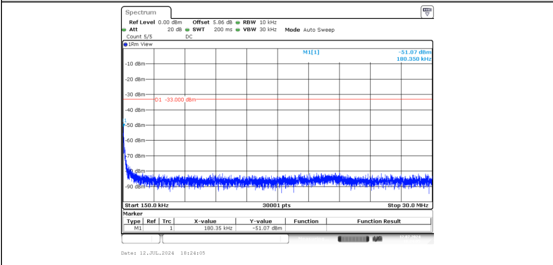
Band2-10MHz-16QAM-18900-1-0-Low-0.15-30--51.07-PASS
