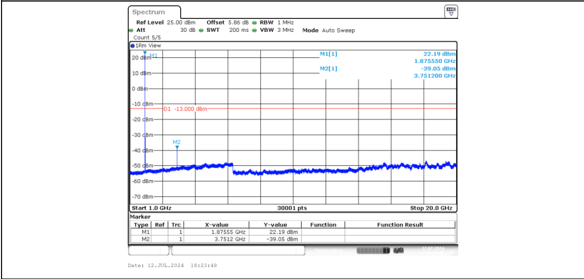
Band2-10MHz-QPSK-18900-1-0-Low-1000-20000--39.05-PASS
