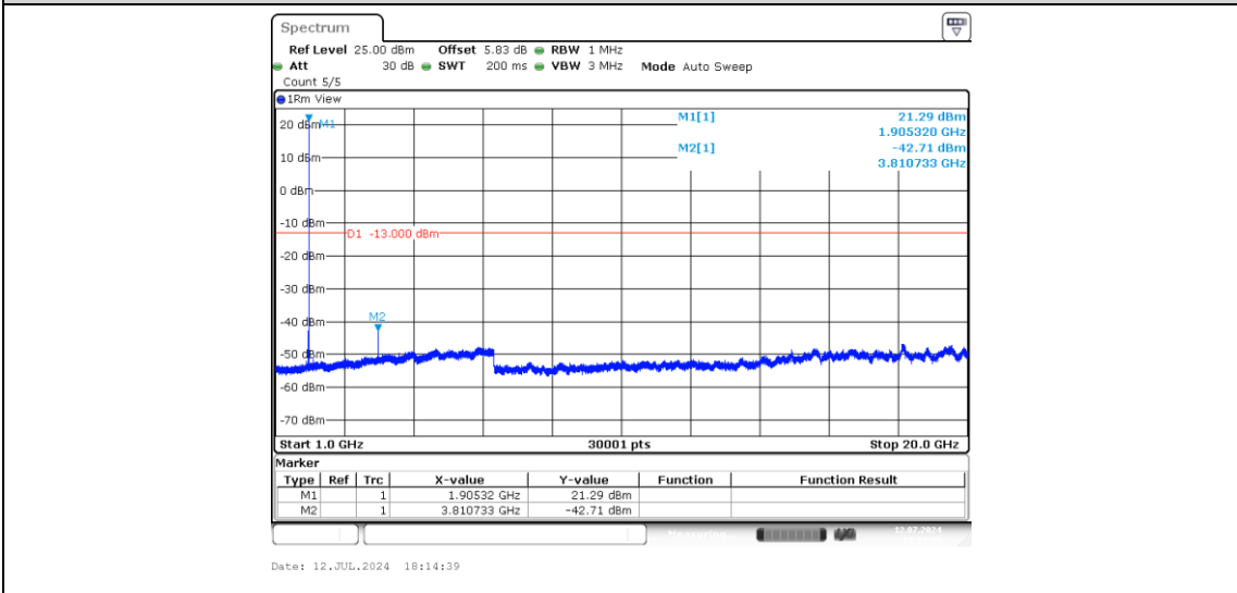
Band2-5MHz-16QAM-19175-1-0-High-1000-20000--42.71-PASS
