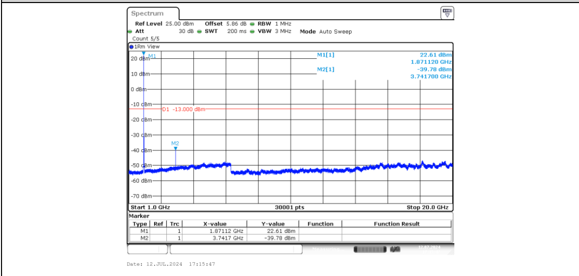
Band2-20MHz-QPSK-18900-1-0-Low-1000-20000--39.78-PASS
