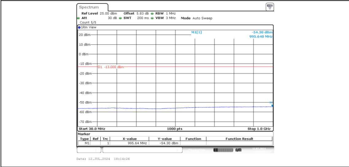
Band2-5MHz-16QAM-19175-1-0-High-30-1000--54.3-PASS
