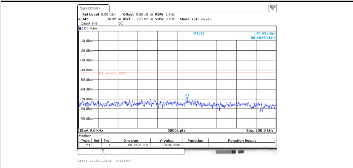
Band2-10MHz-16QAM-18900-1-0-Low-0.009-0.15--70.42-PASS
