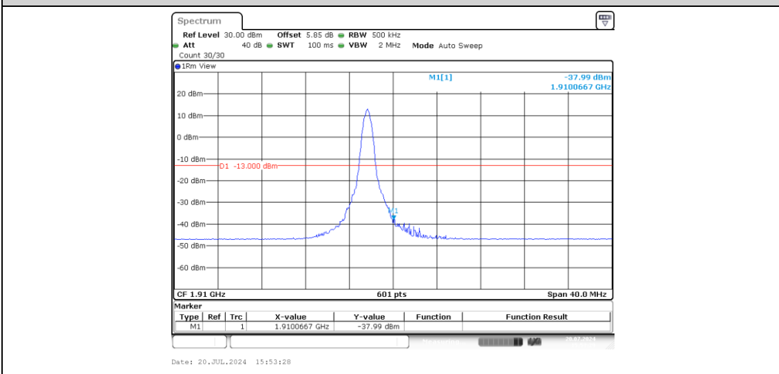
Band2-20MHz-QPSK-19100-1-0-High--37.99-PASS
