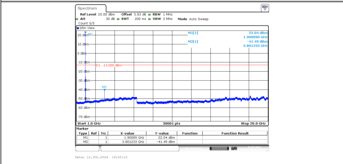
Band2-10MHz-QPSK-19150-1-0-High-1000-20000--41.49-PASS
