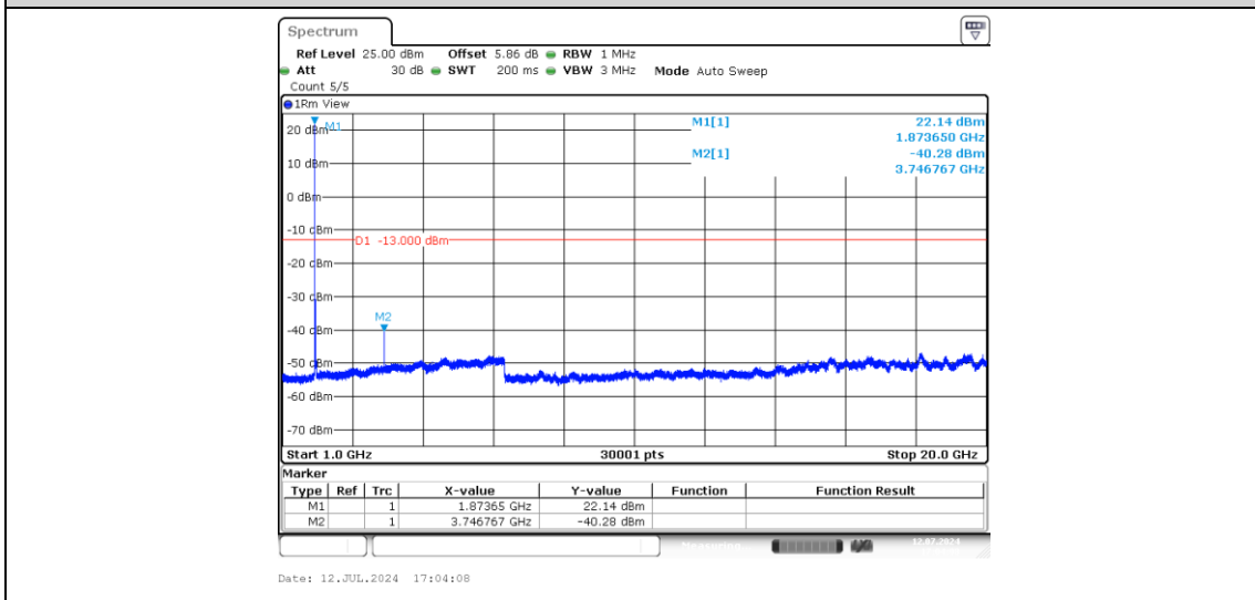
Band2-15MHz-QPSK-18900-1-0-Low-1000-20000--40.28-PASS
