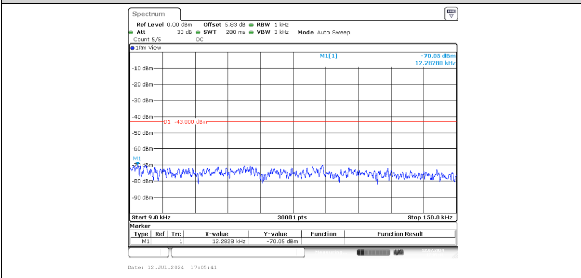
Band2-15MHz-16QAM-19125-1-0-High-0.009-0.15--70.05-PASS
