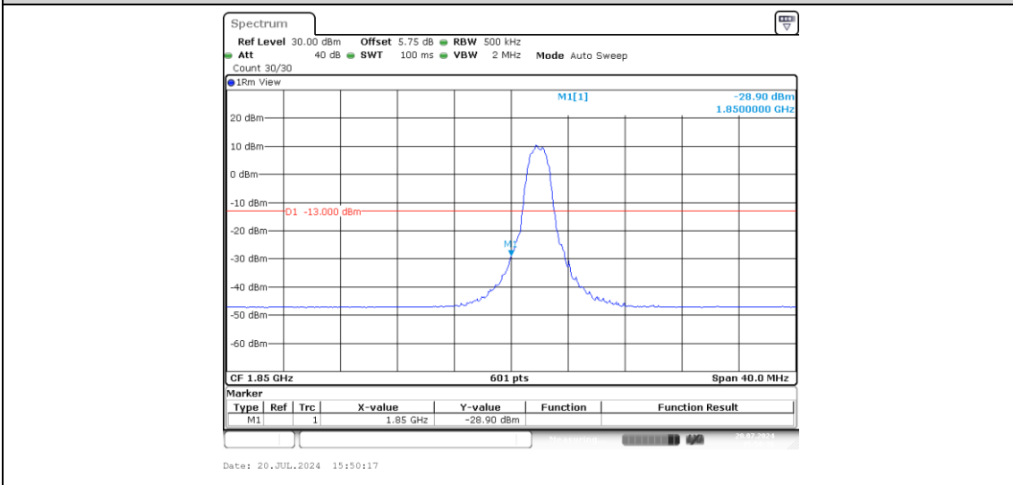
Band2-20MHz-QPSK-18700-6-0-Low--28.90-PASS
