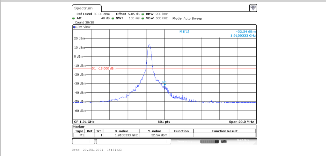
Band2-10MHz-QPSK-19150-1-0-High--32.54-PASS
