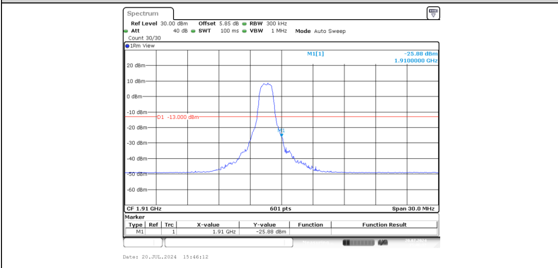
Band2-15MHz-16QAM-19125-6-0-High--25.88-PASS
