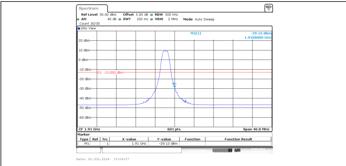
Band2-20MHz-QPSK-19100-6-0-High--29.13-PASS
