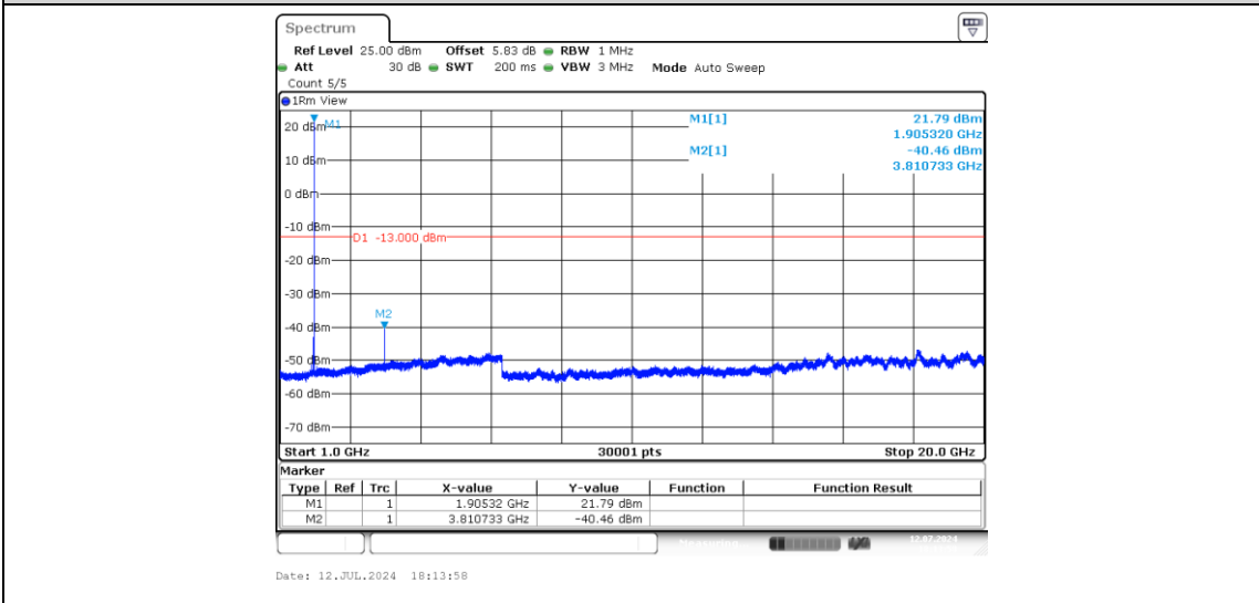
Band2-5MHz-QPSK-19175-1-0-High-1000-20000--40.46-PASS
