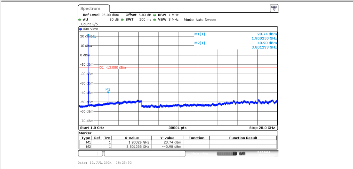
Band2-10MHz-16QAM-19150-1-0-High-1000-20000--40.9-PASS
