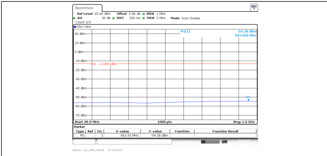
Band2-15MHz-QPSK-18900-1-0-Low-30-1000--54.28-PASS
