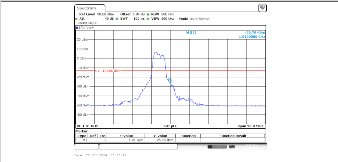
Band2-10MHz-QPSK-19150-6-0-High--26.78-PASS
