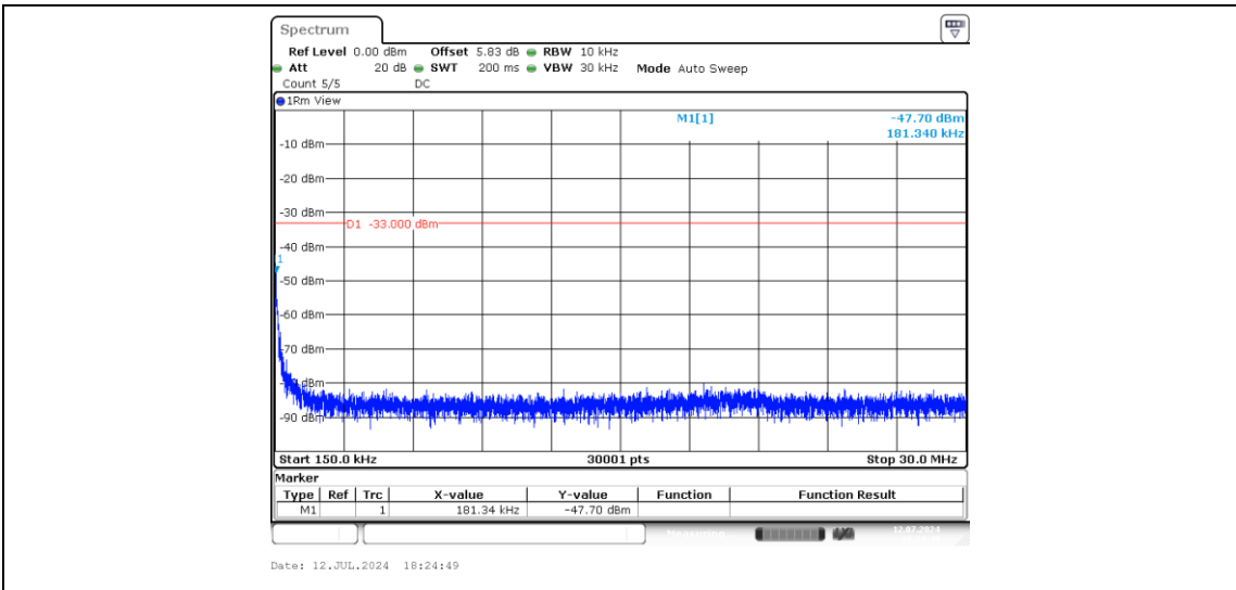
Band2-10MHz-QPSK-19150-1-0-High-0.15-30--47.7-PASS
