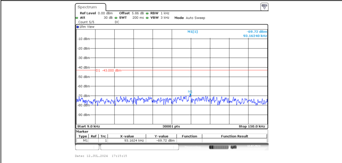
Band2-20MHz-QPSK-18900-1-0-Low-0.009-0.15--69.72-PASS
