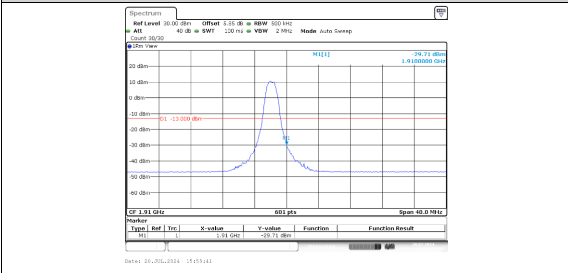
Band2-20MHz-16QAM-19100-6-0-High--29.71-PASS
