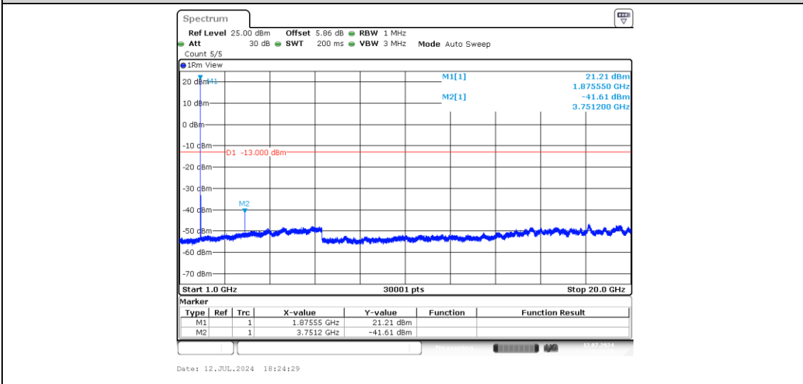
Band2-10MHz-16QAM-18900-1-0-Low-1000-20000--41.61-PASS
