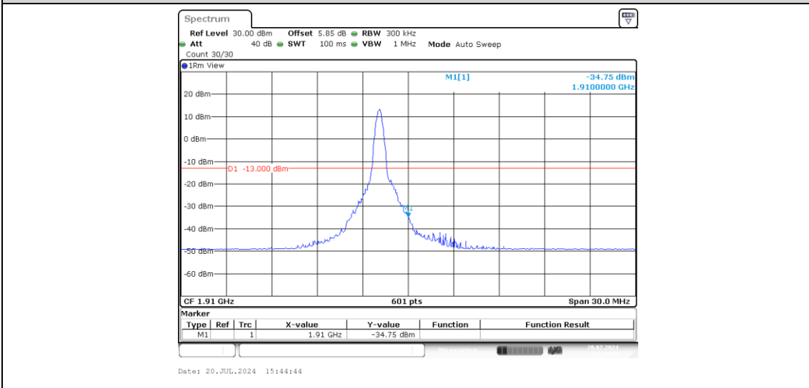
Band2-15MHz-16QAM-19125-1-0-High--34.75-PASS
