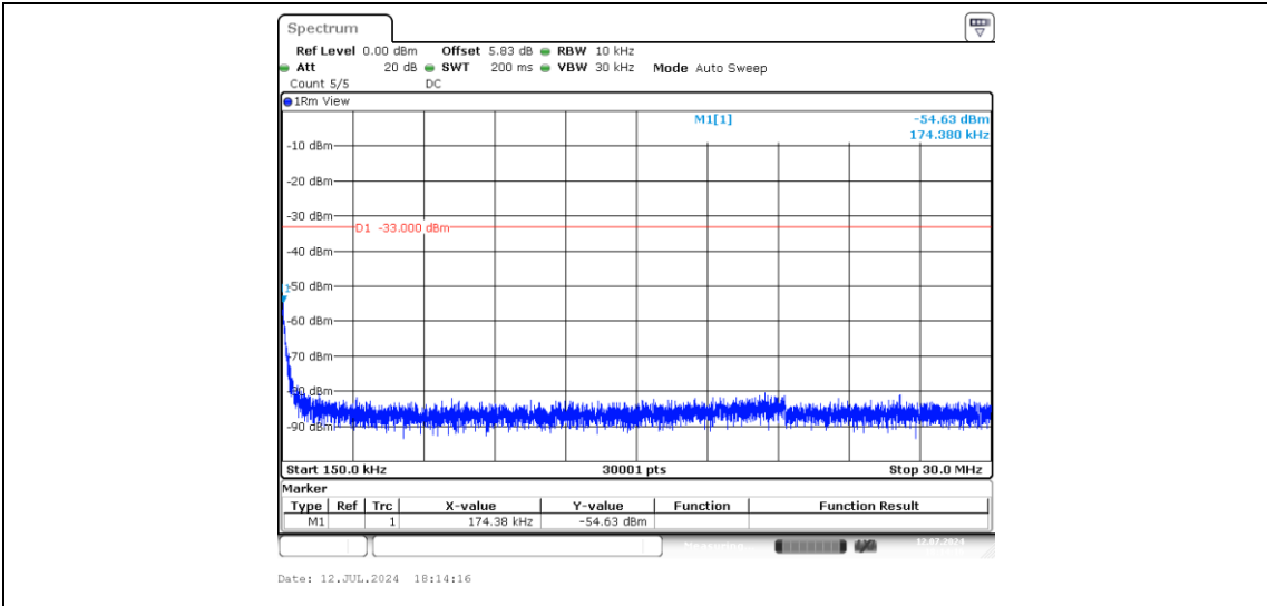
Band2-5MHz-16QAM-19175-1-0-High-0.15-30--54.63-PASS
