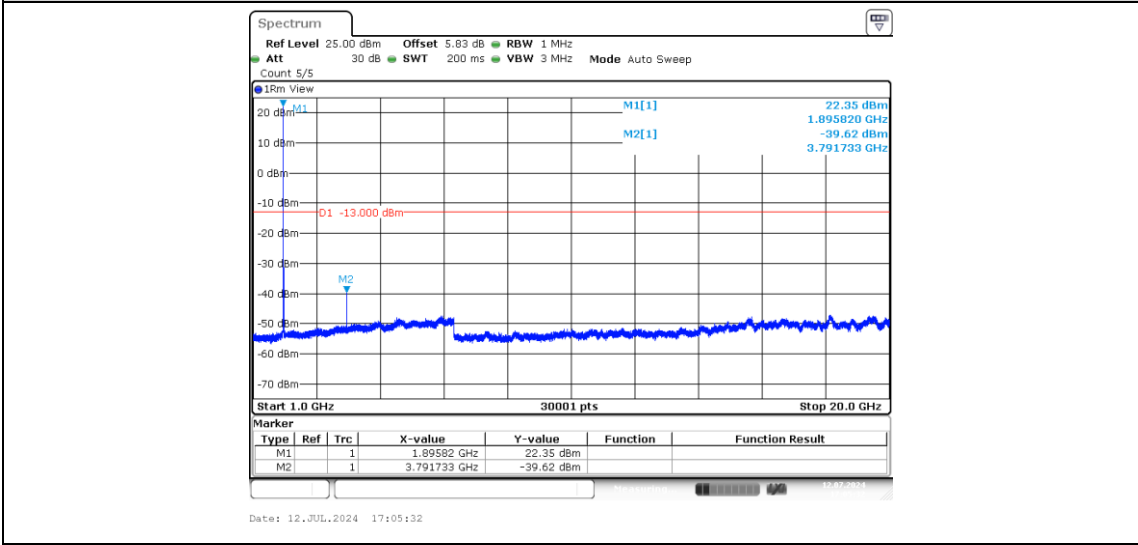
Band2-15MHz-QPSK-19125-1-0-High-1000-20000--39.62-PASS
