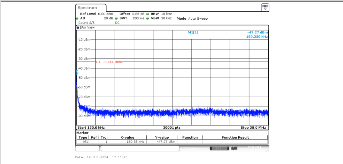
Band2-20MHz-QPSK-18900-1-0-Low-0.15-30--47.27-PASS
