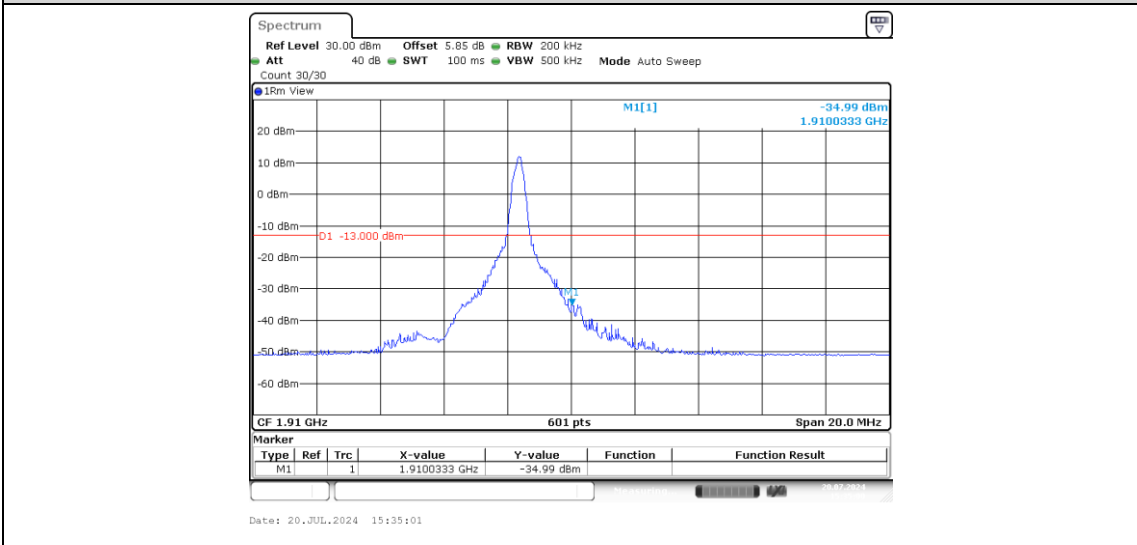
Band2-10MHz-16QAM-19150-1-0-High--34.99-PASS
