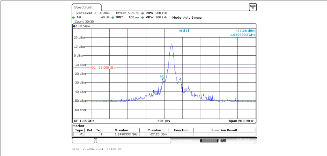
Band2-10MHz-16QAM-18650-1-0-Low--27.26-PASS
