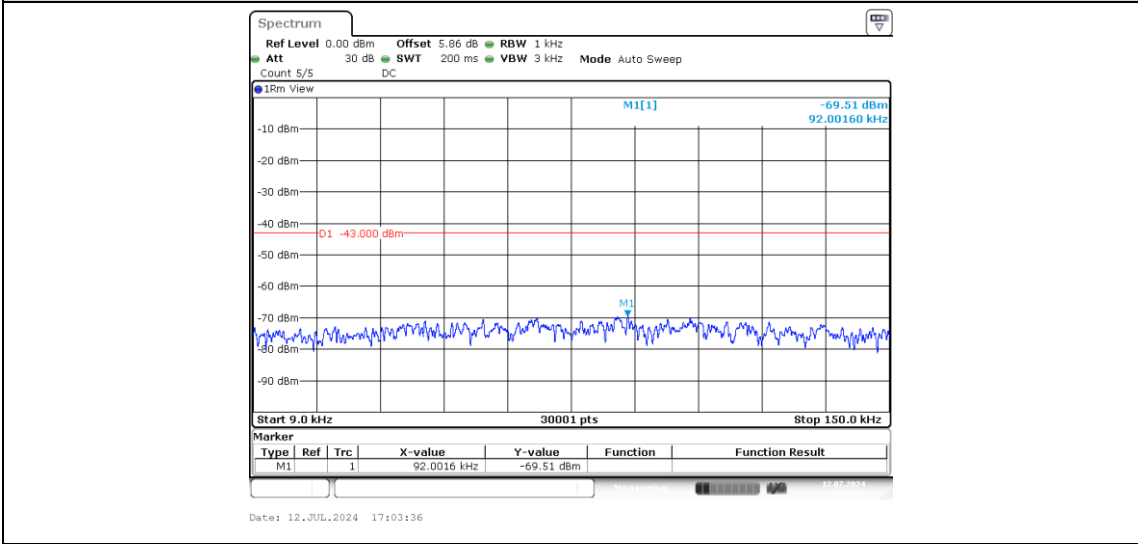
Band2-15MHz-QPSK-18900-1-0-Low-0.009-0.15--69.51-PASS
