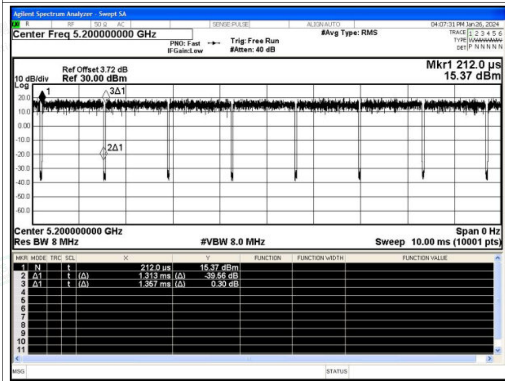
Duty Cycle NVNT ax20 5200MHz Ant0
