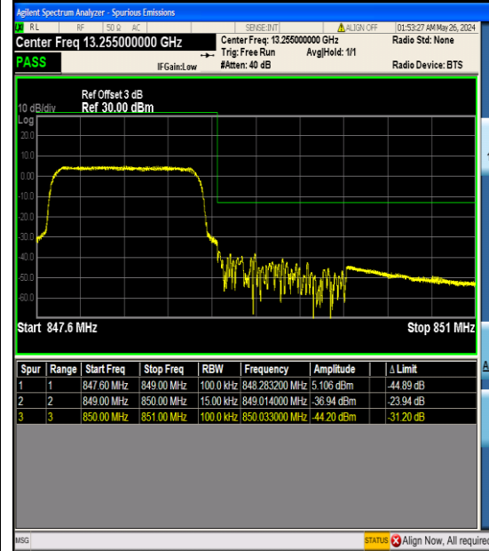
Band26_1.4MHz_QPSK_27033_6RB#0
