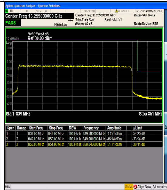
Band26_10MHz_16QAM_26990_50RB#0
