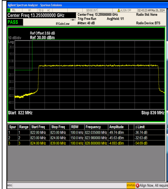
Band26_15MHz_QPSK_26865_75RB#0
