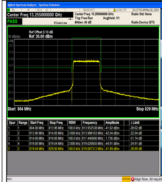
Band26_5MHz_16QAM_26715_25RB#0
