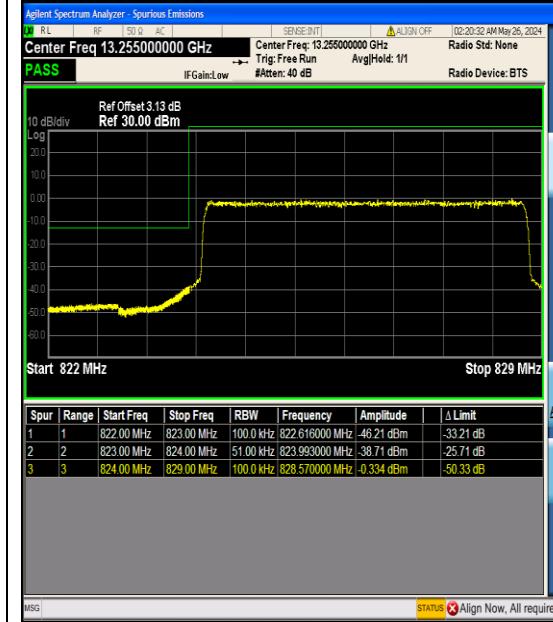
Band26_5MHz_QPSK_26815_25RB#0
