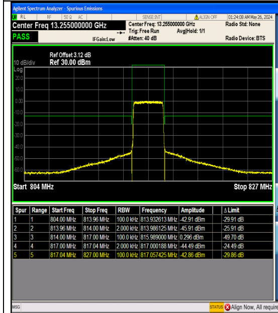
Band26_3MHz_16QAM_26705_15RB#0
