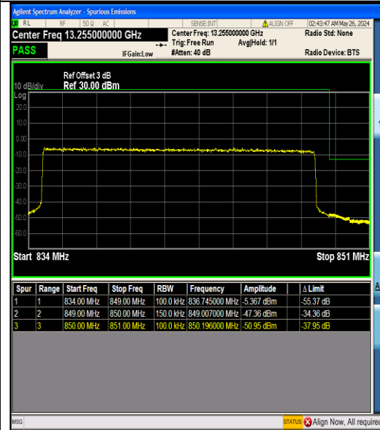
Band26_15MHz_QPSK_26965_75RB#0
