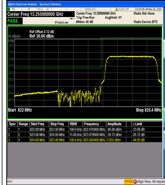
Band26_1.4MHz_QPSK_26797_6RB#0
