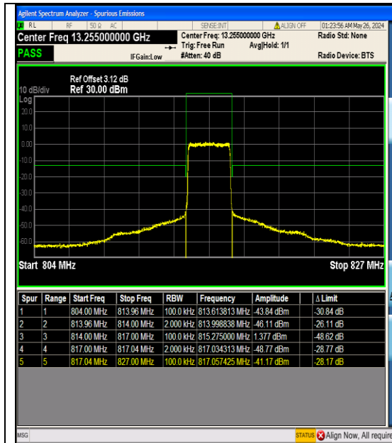
Band26_3MHz_QPSK_26705_15RB#0
