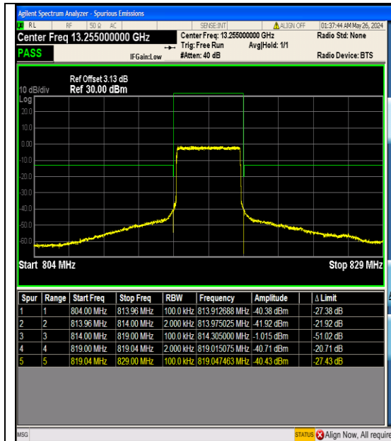
Band26_5MHz_QPSK_26715_25RB#0
