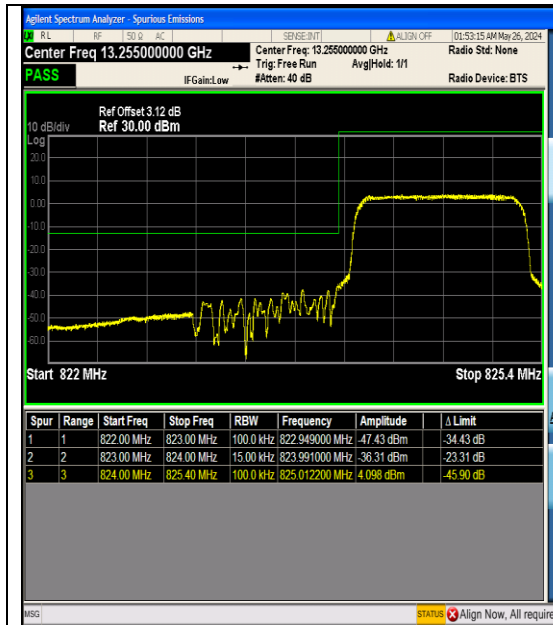
Band26_1.4MHz_16QAM_26797_6RB#0
