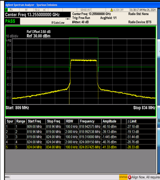
Band26_5MHz_16QAM_26765_25RB#0
