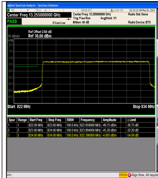
Band26_10MHz_16QAM_26840_50RB#0
