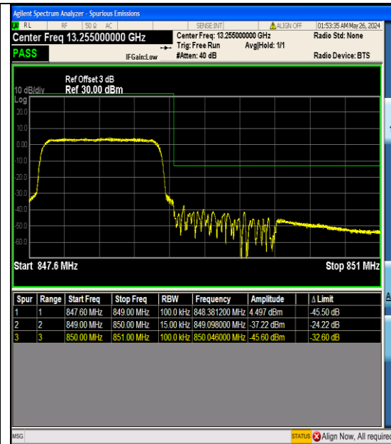
Band26_1.4MHz_16QAM_27033_6RB#0
