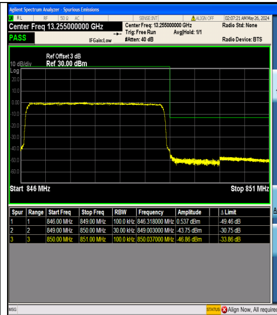
Band26_3MHz_16QAM_27025_15RB#0
