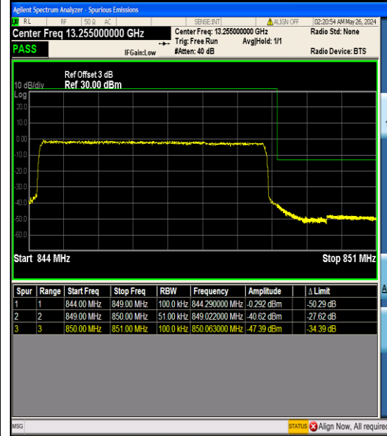
Band26_5MHz_QPSK_27015_25RB#0
