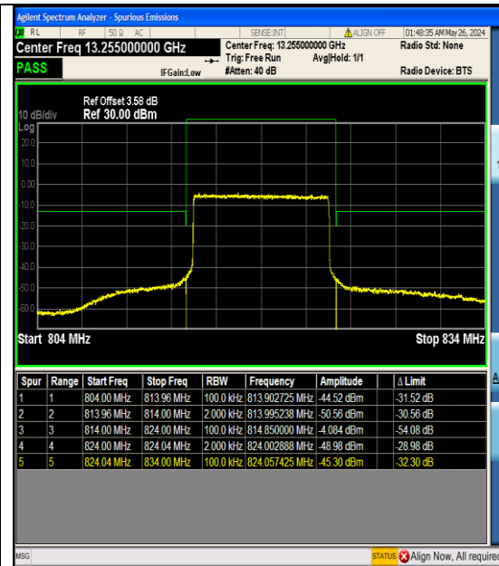
Band26_10MHz_16QAM_26740_50RB#0
