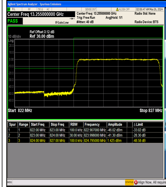
Band26_3MHz_QPSK_26805_15RB#0
