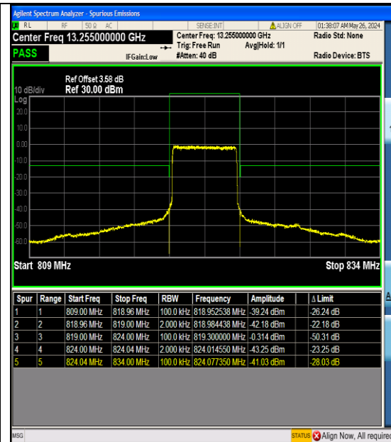
Band26_5MHz_QPSK_26765_25RB#0
