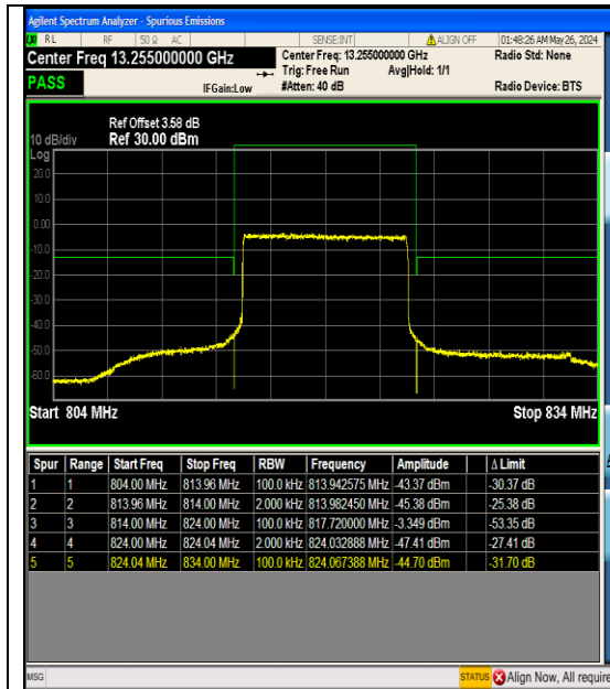
Band26_10MHz_QPSK_26740_50RB#0
