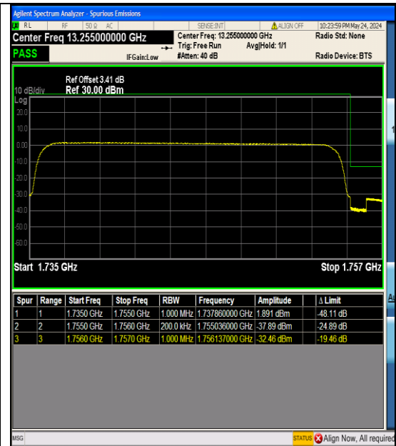
Band4_20MHz_QPSK_20300_100RB#0
