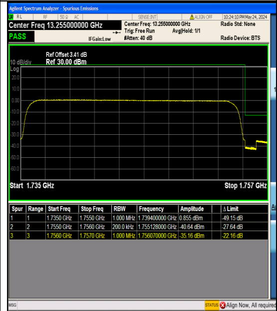
Band4_20MHz_16QAM_20300_100RB#0
