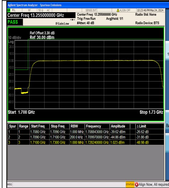
Band4_20MHz_16QAM_20050_100RB#0
