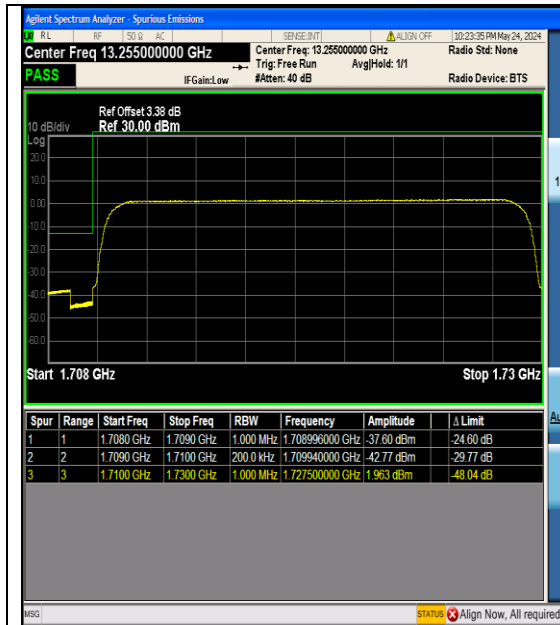
Band4_20MHz_QPSK_20050_100RB#0
