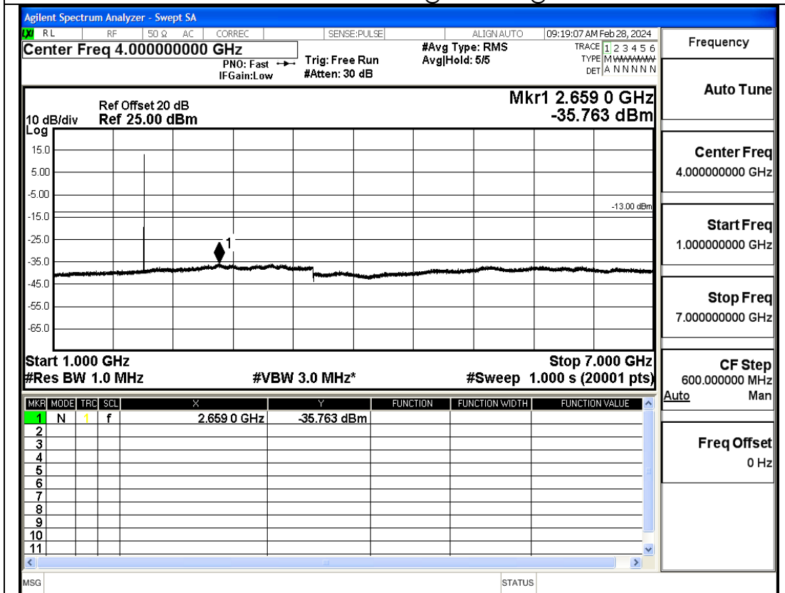
GSM1900-1909.8MHz-Voice@7GHz-13.6GHz@Pass
