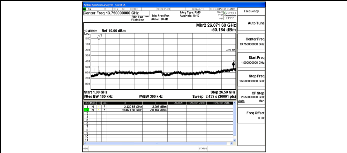
11N20SISO-Ant1-2437-1000~26500-PASS
