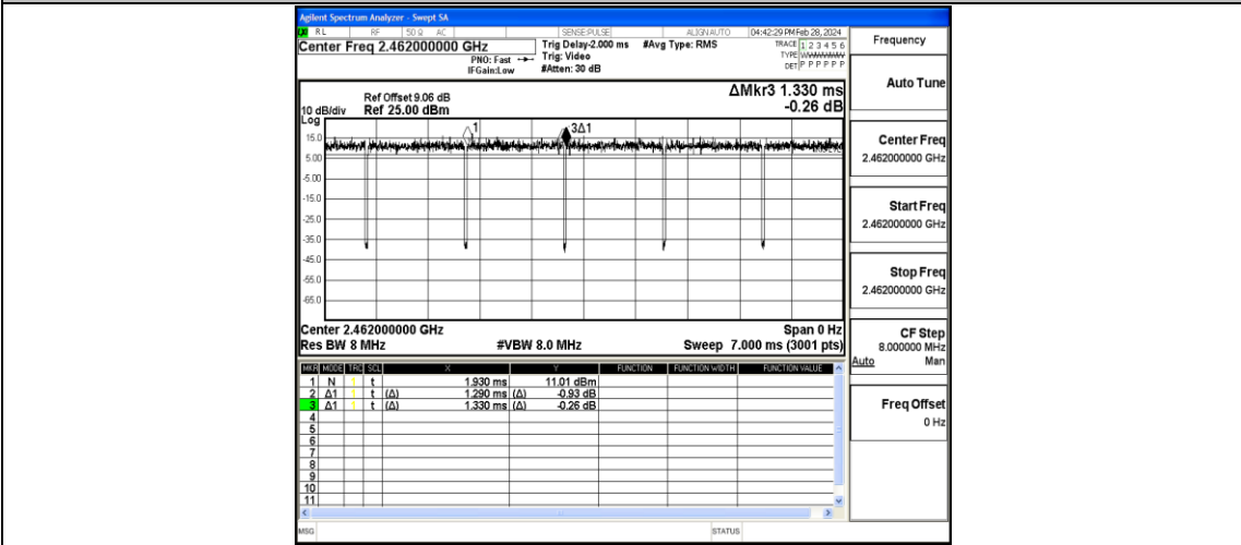
NTVN-11N20SISO-Ant1-2462
