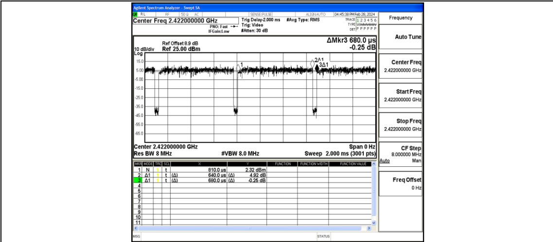
NTVN-11N40SISO-Ant1-2422
