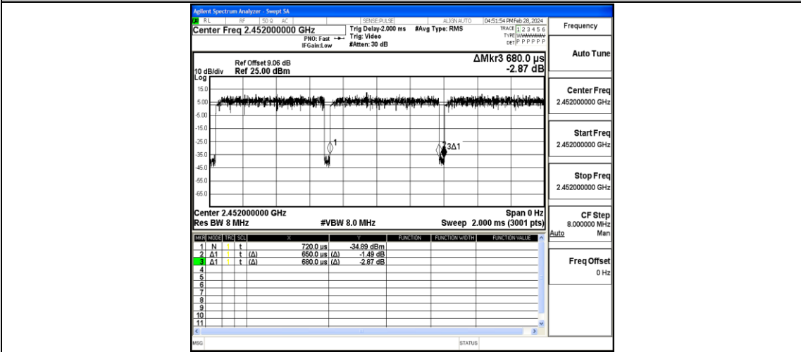
NTVN-11N40SISO-Ant1-2452
