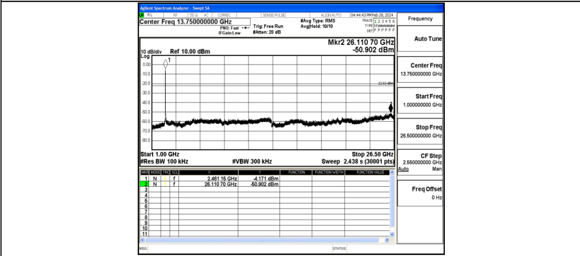
11N20SISO-Ant1-2462-1000~26500-PASS
