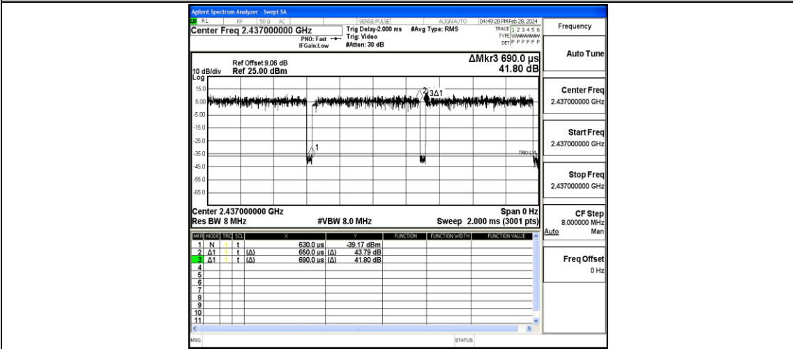
NTVN-11N40SISO-Ant1-2437
