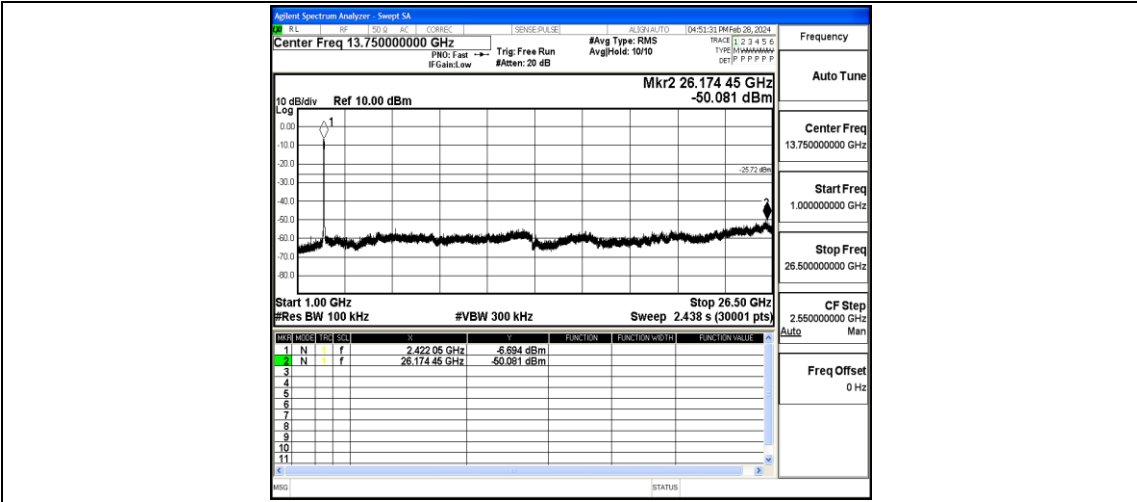
11N40SISO-Ant1-2437-1000~26500-PASS
