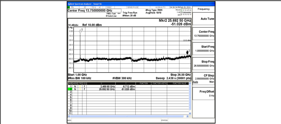
11G-Ant1-2462-1000~26500-PASS
